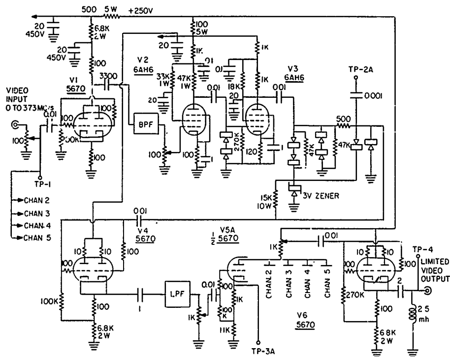
Fig. 3 - Schematic diagram of one channel of the five-channel contiguous filter
