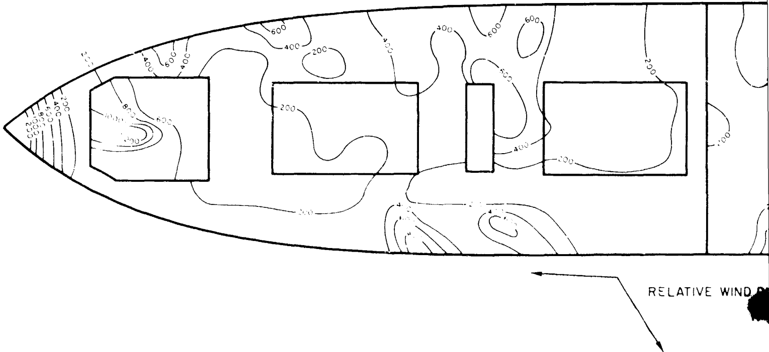
Figure 9.8 Radiation contours
