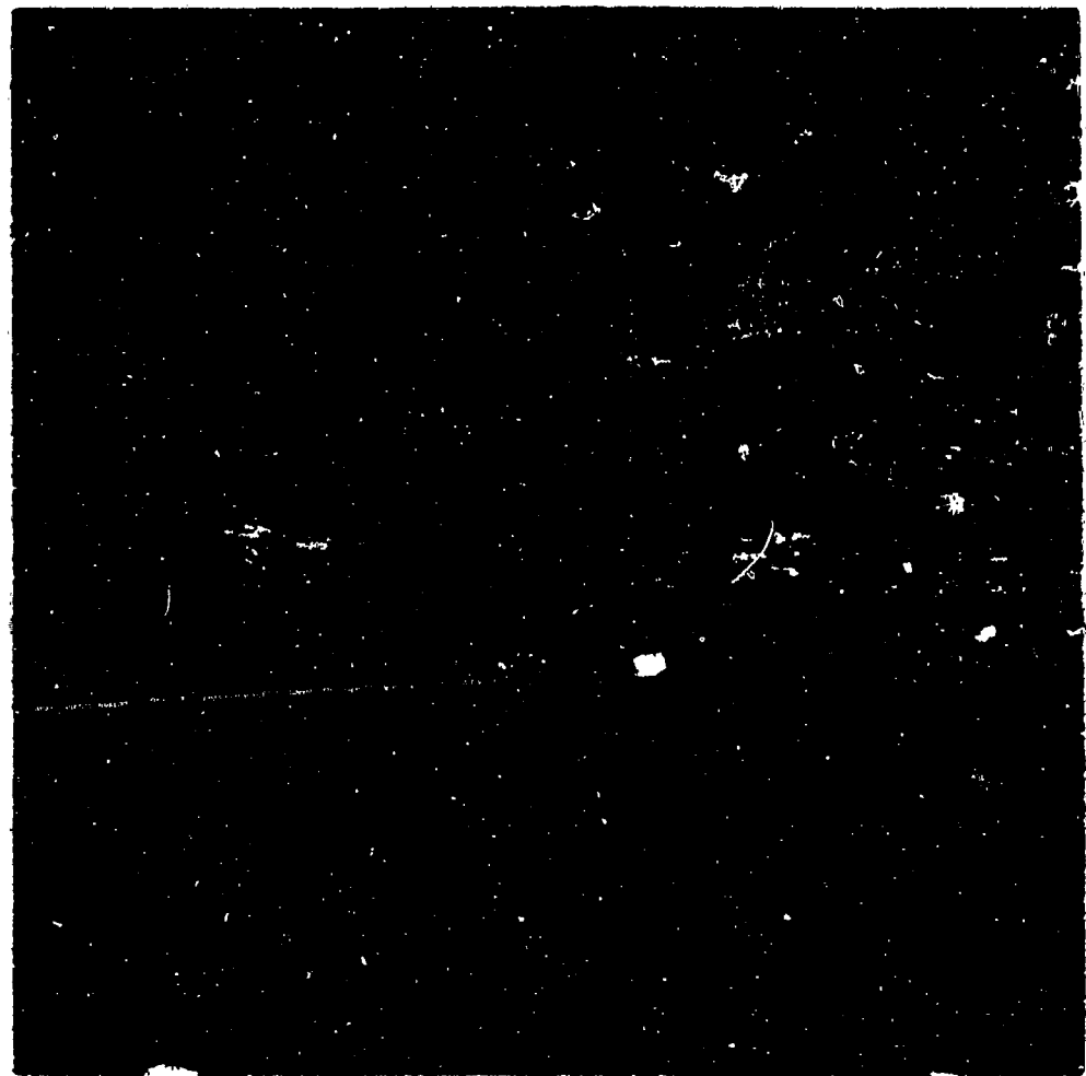
Figure 62. Typical grease streak photograph of flow pattern due to impingement on flat plate. p_1/p_\infty = 3.57 ; x/d_N = 5.32 .
