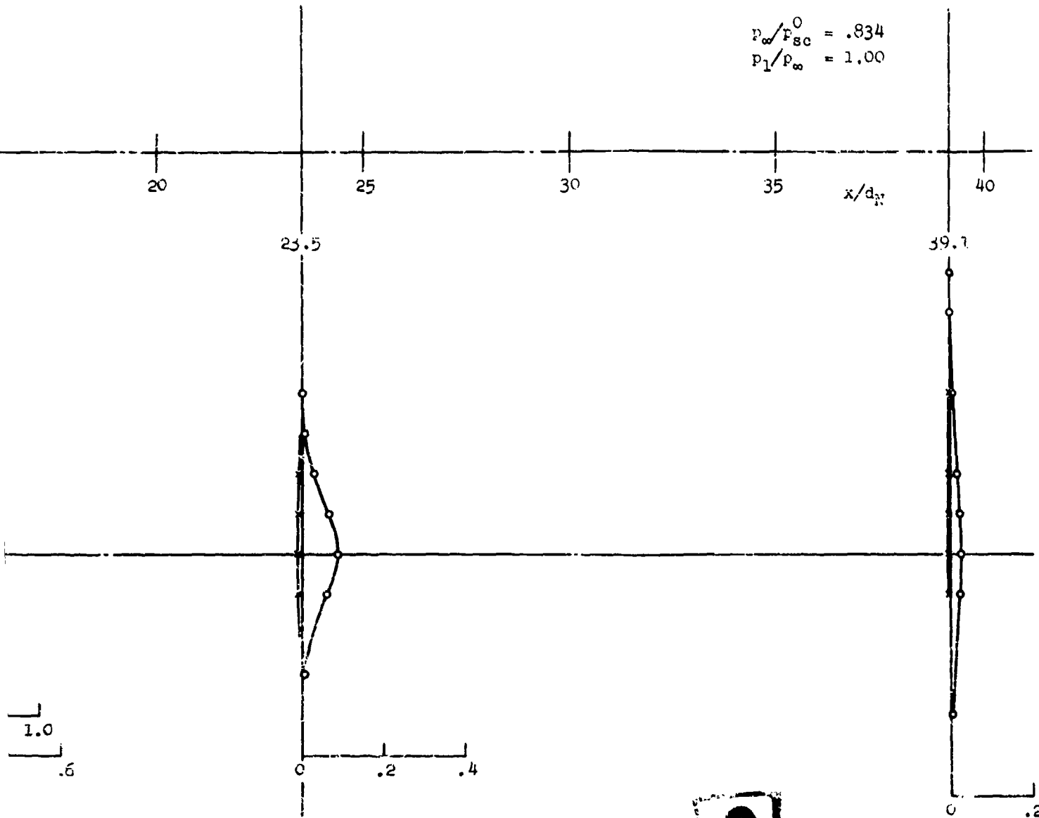
Figure 5. Measured jet total and static pressure distributions.
