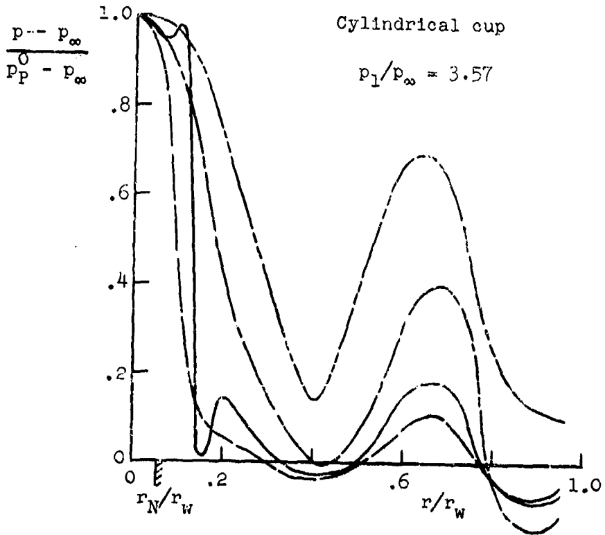
Figure 38. Measured over-all pressure distributions.
