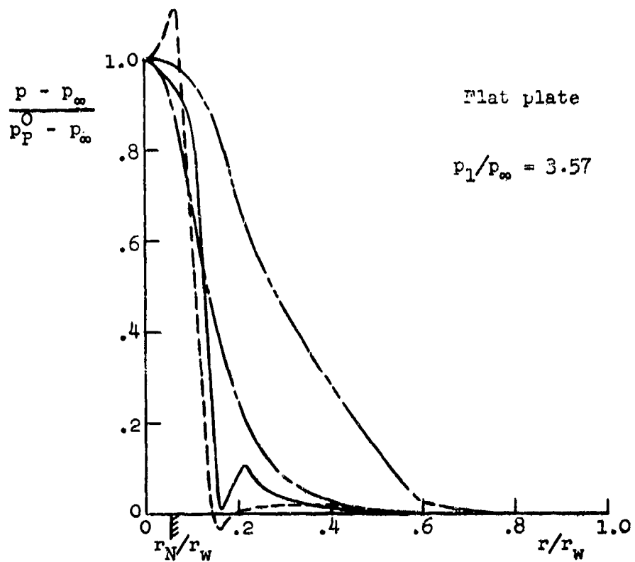
Figure 32. Measured over-all pressure distributions.
