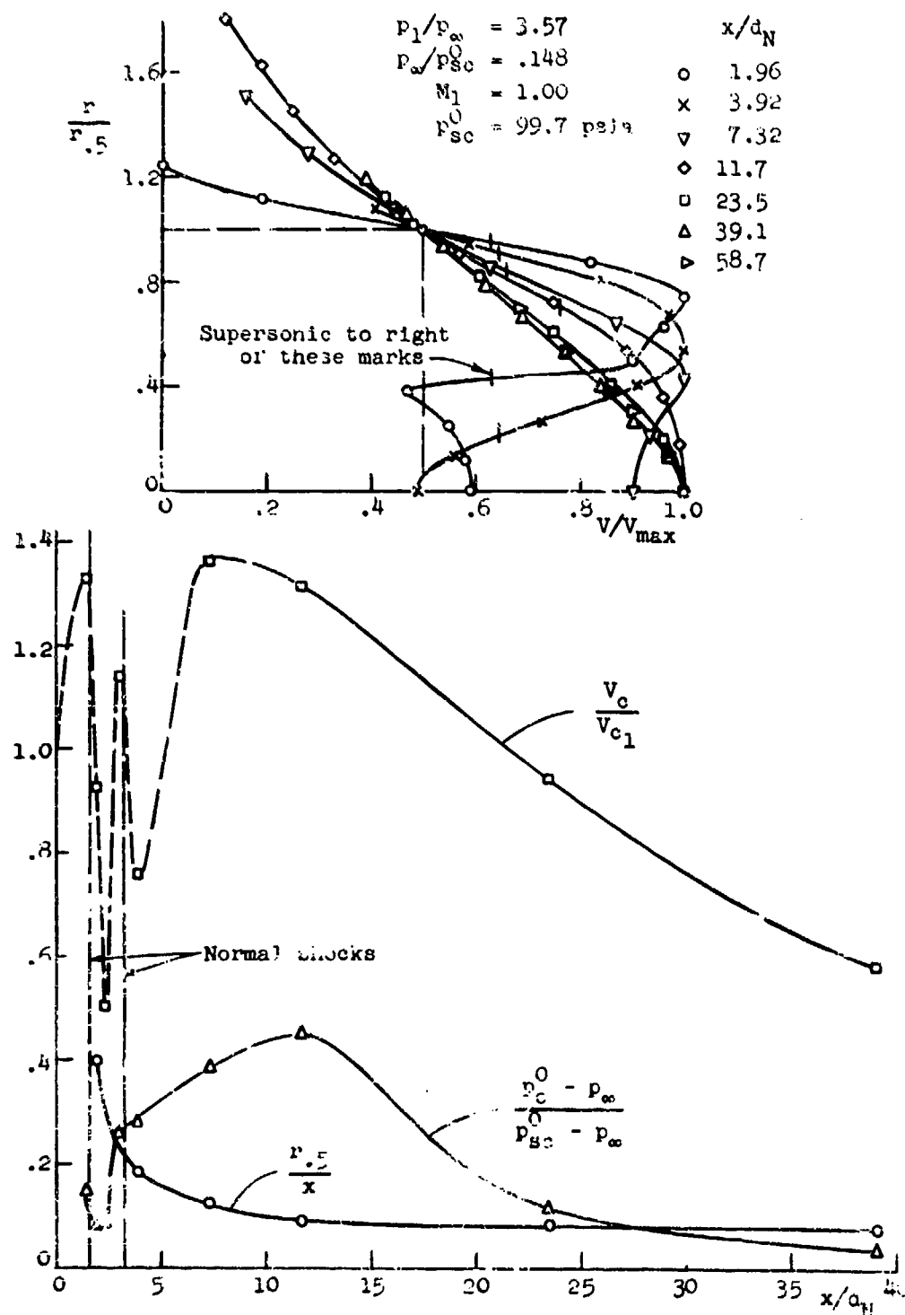
Figure 11. Normalized jet velocity profiles and axial decay and spreading characteristics.
