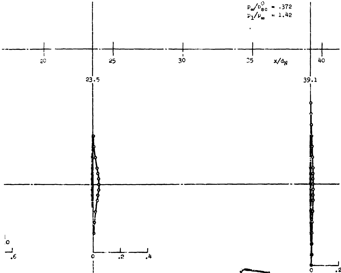
Figure 7. Measured jet total and static pressure distributions.
