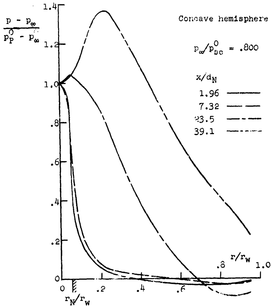
Figure 35. Measured over-all pressure distributions.
