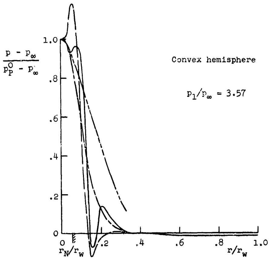
Figure 34. Measured over-all pressure distributions.
