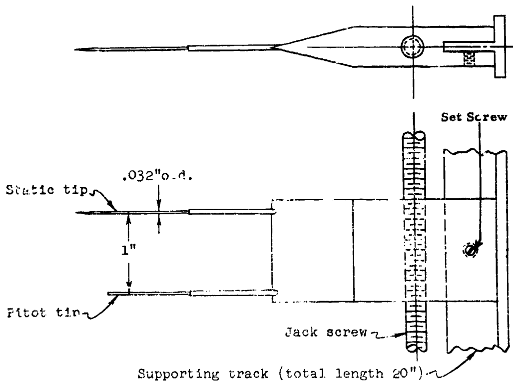
Figure 4. Combination probe used in free jet surveys.
