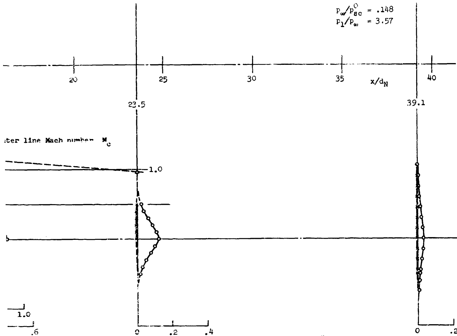
Figure 10. Measured jet total and static pressure distributions.
