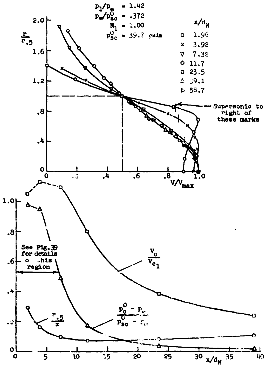
Figure 8. Normalized jet velocity profiles and axial decay and spreading characteristics.
