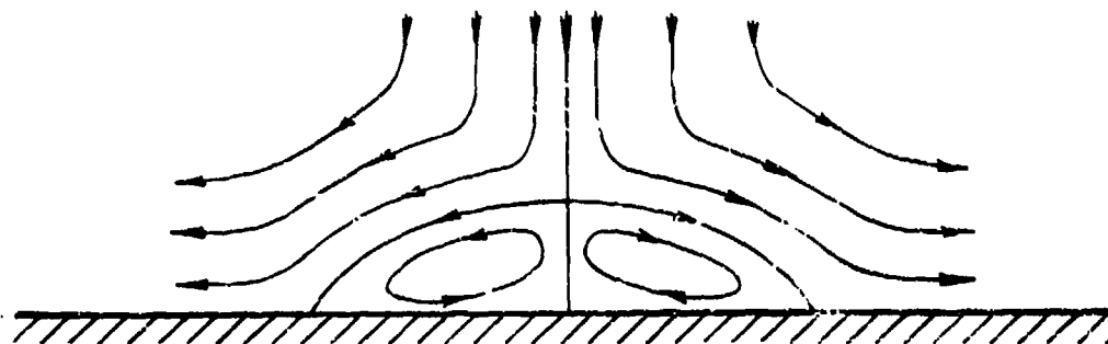
Figure 60. Flow pattern of separated region (distance normal to surface exaggerated).
