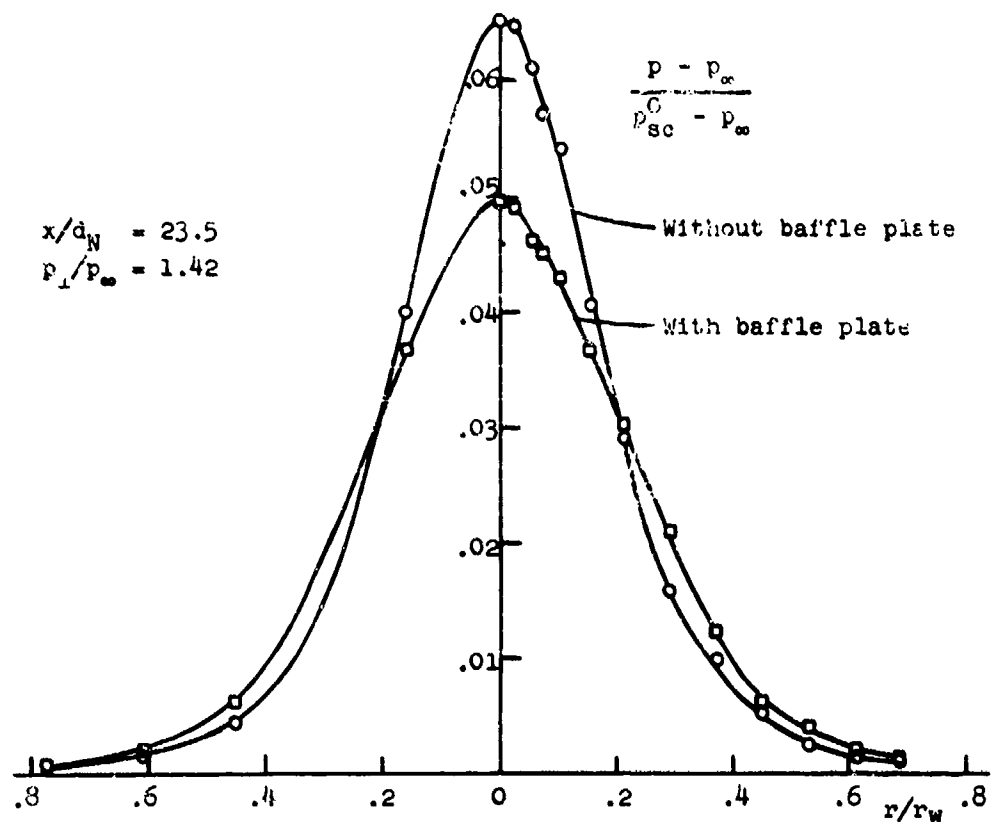
Figure 63. Example of changes in impingement pressure distribution due to baffle plate.
