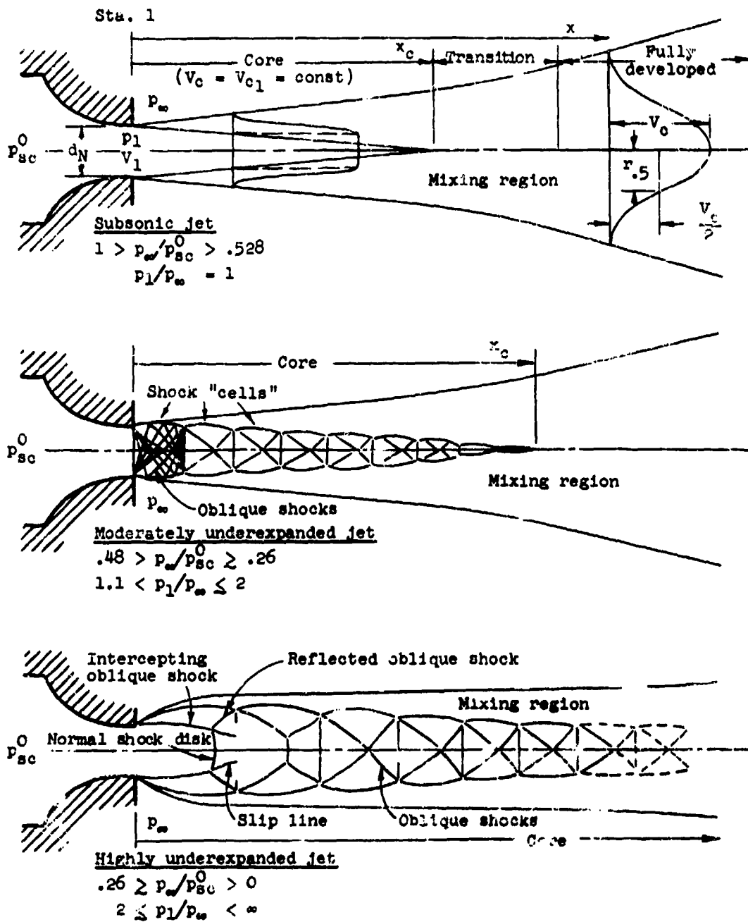
Figure 1. Three major variations of jet flow from a sonic nozzle.
