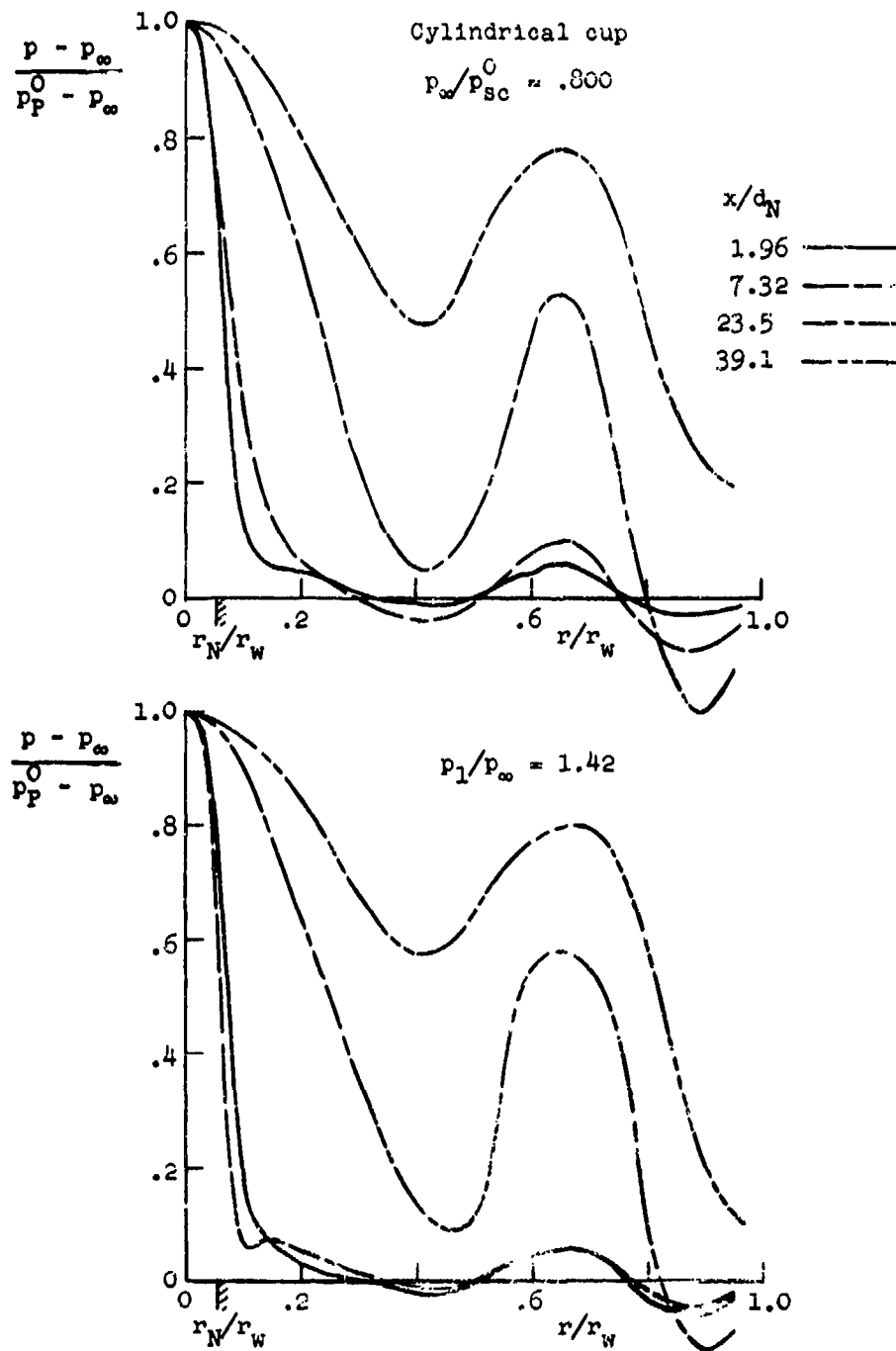
Figure 37. Measured over-all pressure distributions.
