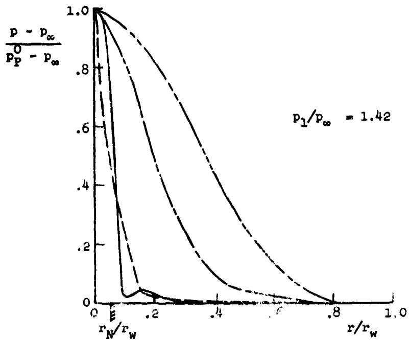
Figure 31. Measured over-all pressure distributions.
