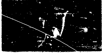
Figure 43. Schlieren pictures of impingement on flat plate at x/d_N = 1.96 . Knife edge horizontal.
