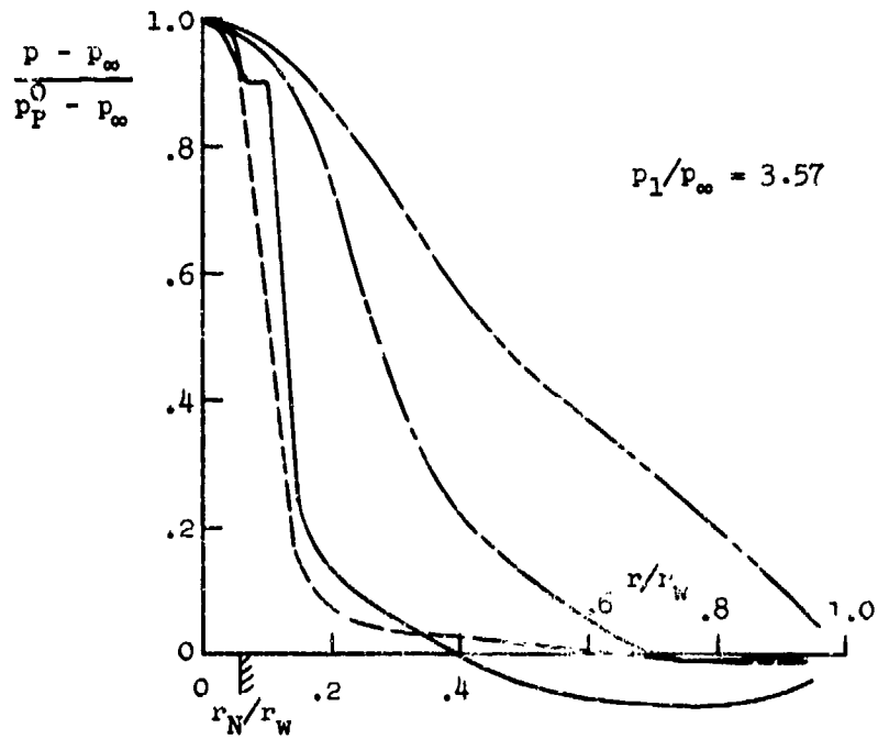
Figure 36. Measured over-all pressure distributions.
