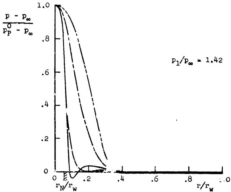
Figure 33. Measured over-all pressure distributions.
