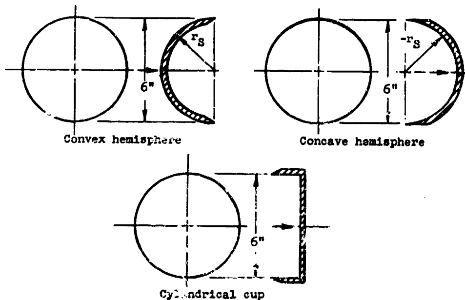
Figure 17. Basic impingement model shapes.
