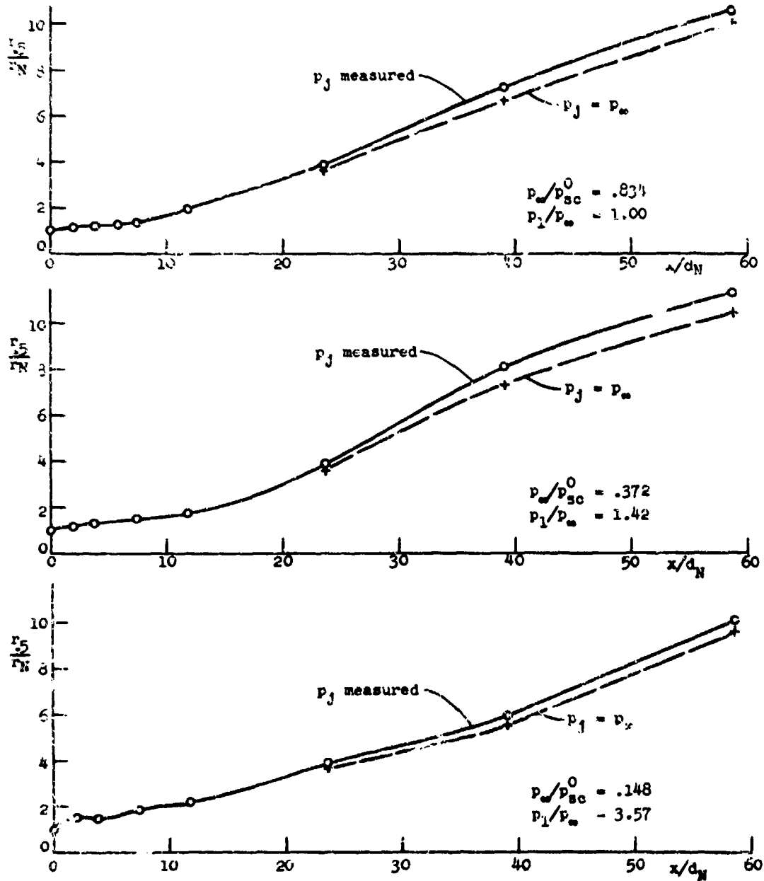
Figure 12. Measured radial spread of subsonic and underexpanded free jets.
