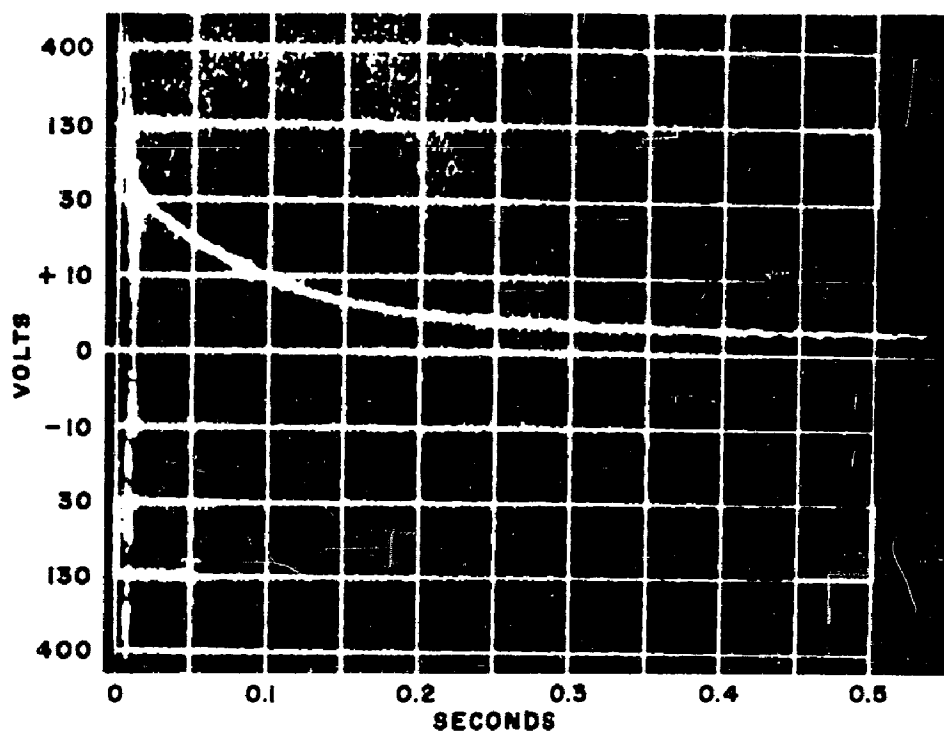
Figure 3.15 Line-to-ground potential.
