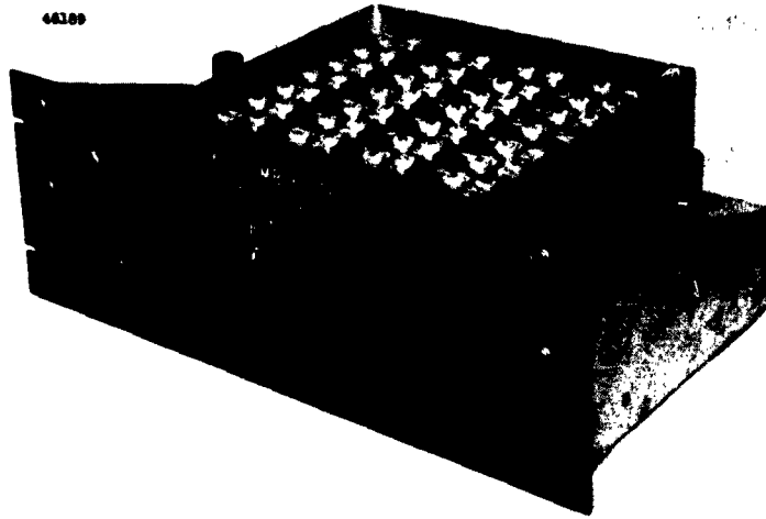
Fig. 2 - Single bank, cover removed, trimmers shown
