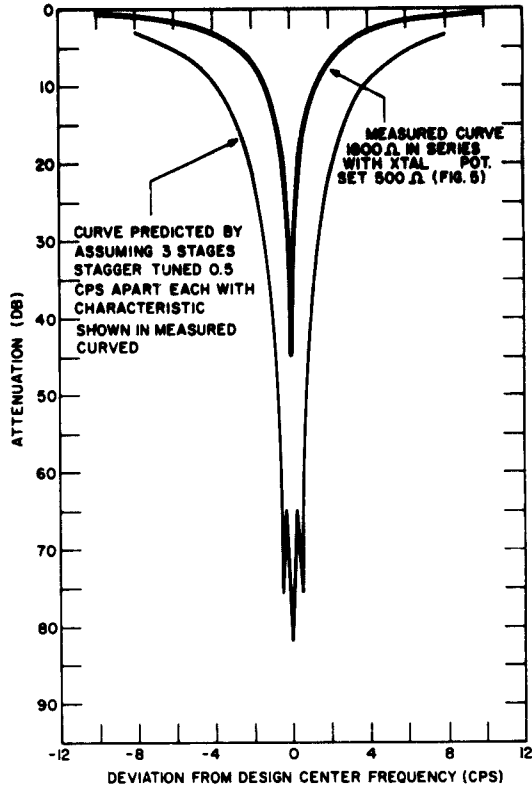
Fig. 6 - Single null characteristic and predicted three-section bank characteristic
