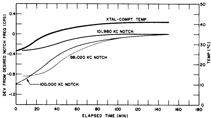
Fig. 15 - Notch frequency and crystal-compartment temperature vs warmup time
