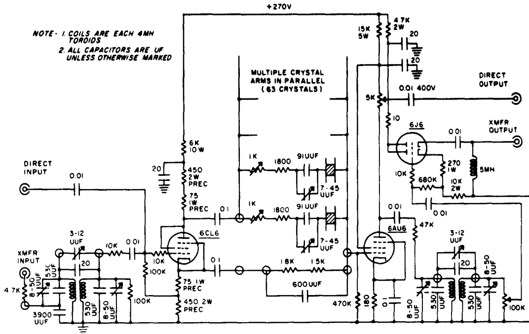
Fig. 5 - Schematic diagram of one bank of 100-kc crystal comb filter
