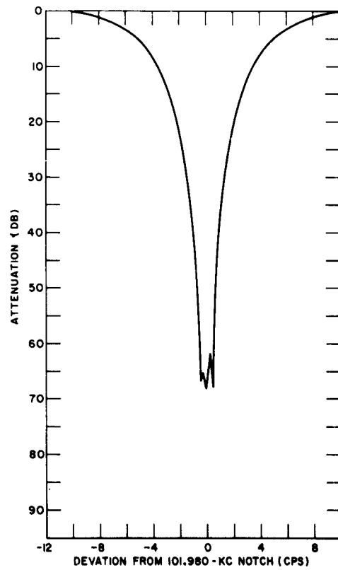
Fig. 9 - Measured three-bank, single-notch response at 101.980 kc for cw input
