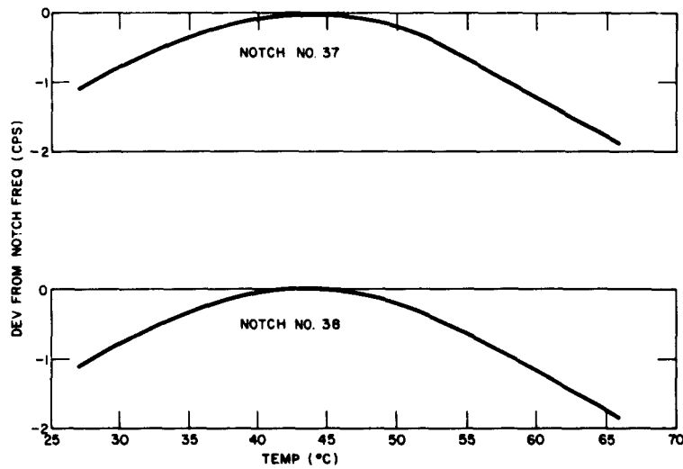
Fig. 14 - Crystal-frequency change vs temperature for two typical units
