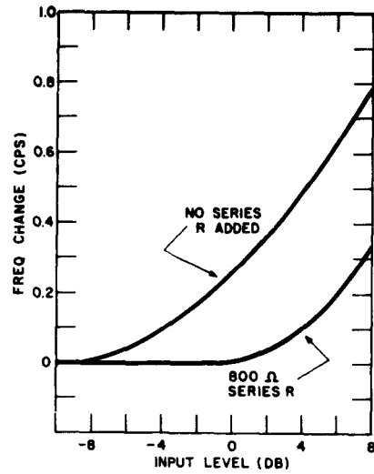
Fig. 13 - Crystal-frequency change vs input level for G-9 crystal unit
