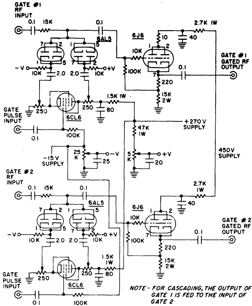
Fig. 18 - Schematic diagram of two-stage gate
