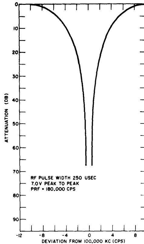
Fig. 19 - Overall three-bank filter response to a pulsed rf input signal
