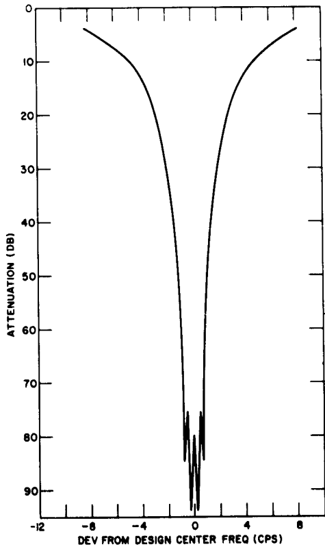
Fig. 7 - Predicted four-bank characteristic
