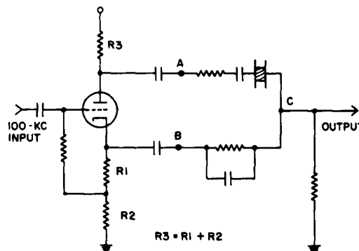
Fig. 4 - Simplified schematic of crystal bridge circuit for attenuation characteristic
