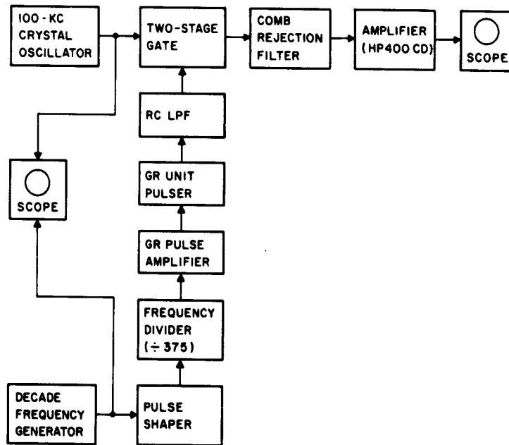
Fig. 17 - Block diagram of instrumentation for determining overall three-bank filter response to a pulsed rf input signal
