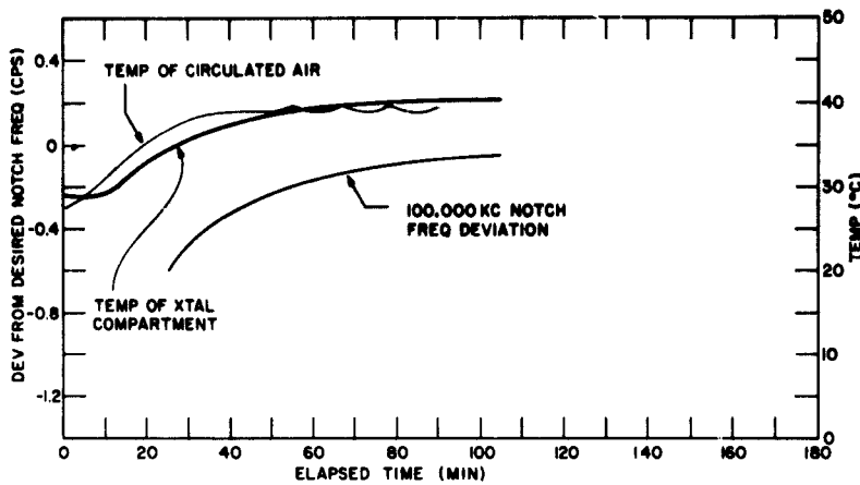
Fig. 16 - Notch frequency and temperature of air circulated in rack vs warmup time
