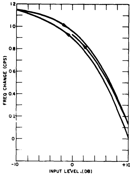
Fig. 12 - Crystal-frequency change vs input level for H-17 crystal unit
