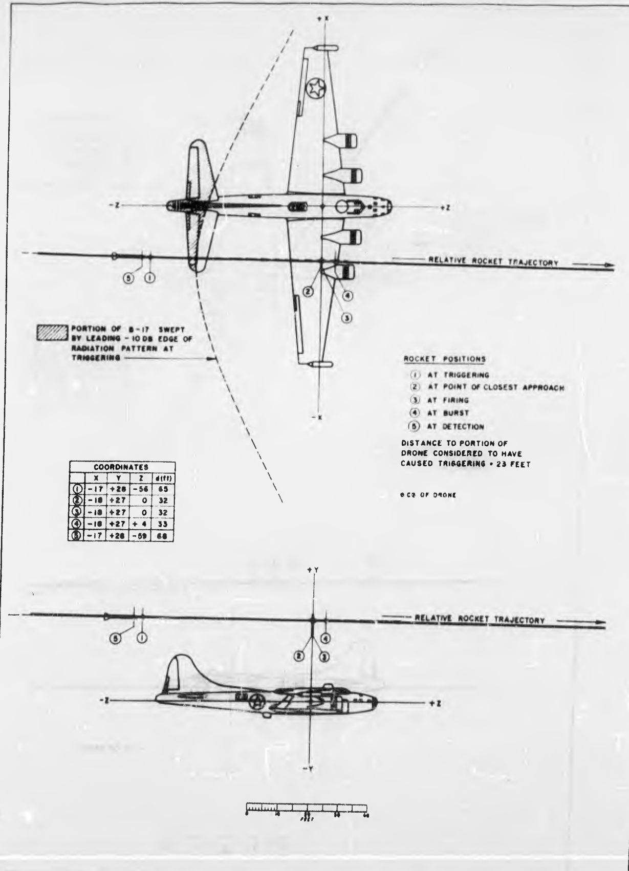
Interception of B-17 Drone by Fuze T2060, S/N B-17. Flight on 29 April 1955. Bird Dog R/N 66. Figure 4.
