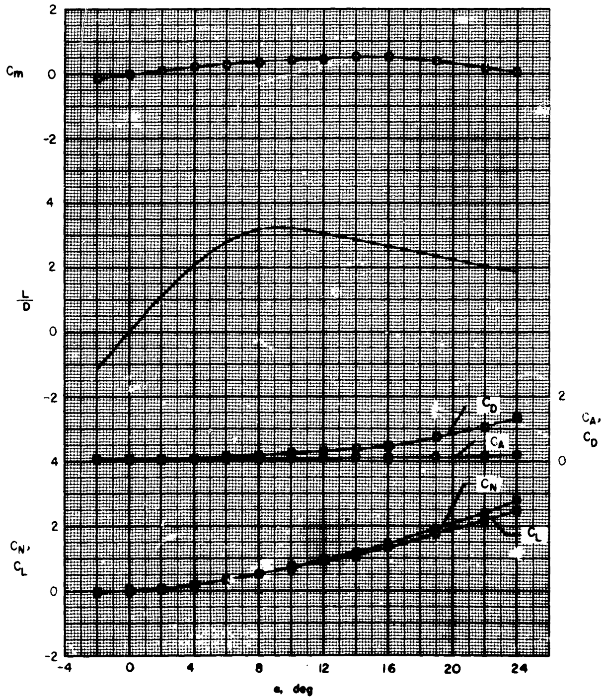
Figure 2.- Aerodynamic characteristics in pitch for body alone.
