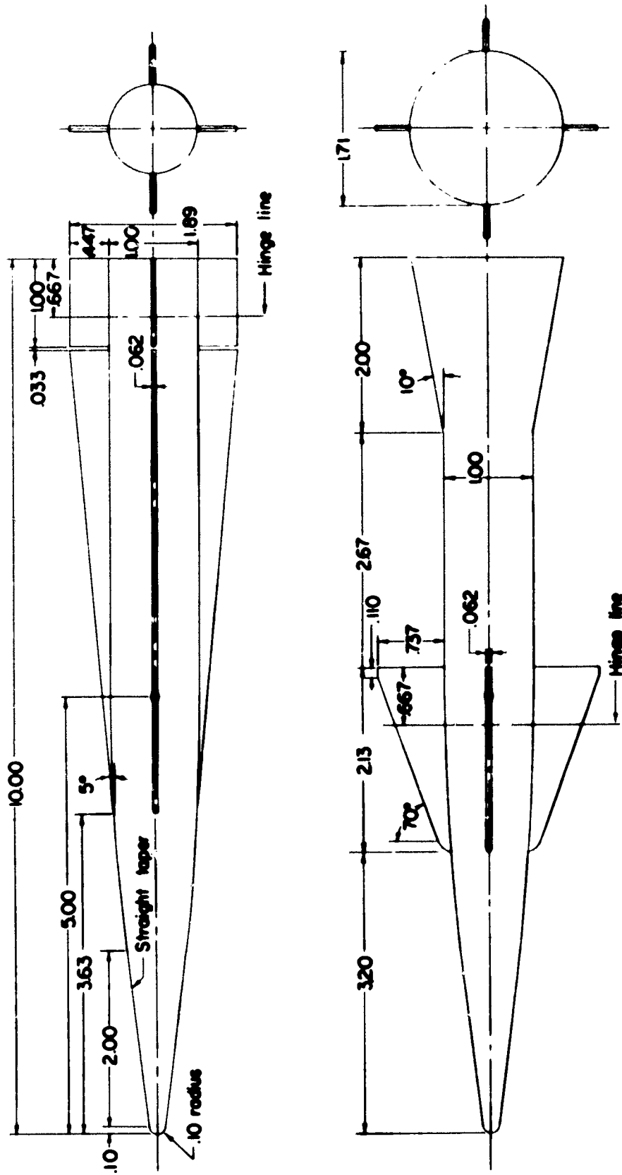
Figure 1.- Details of models. All linear dimensions are in calibers.
