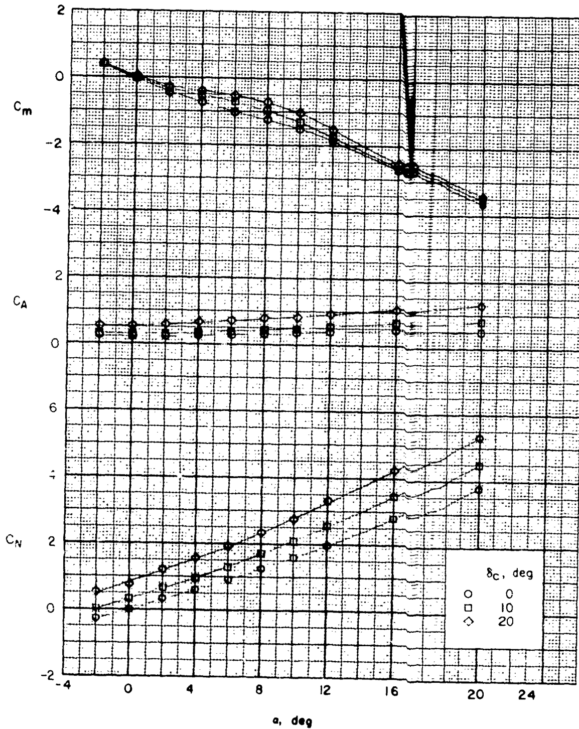
(a) Body axis.
