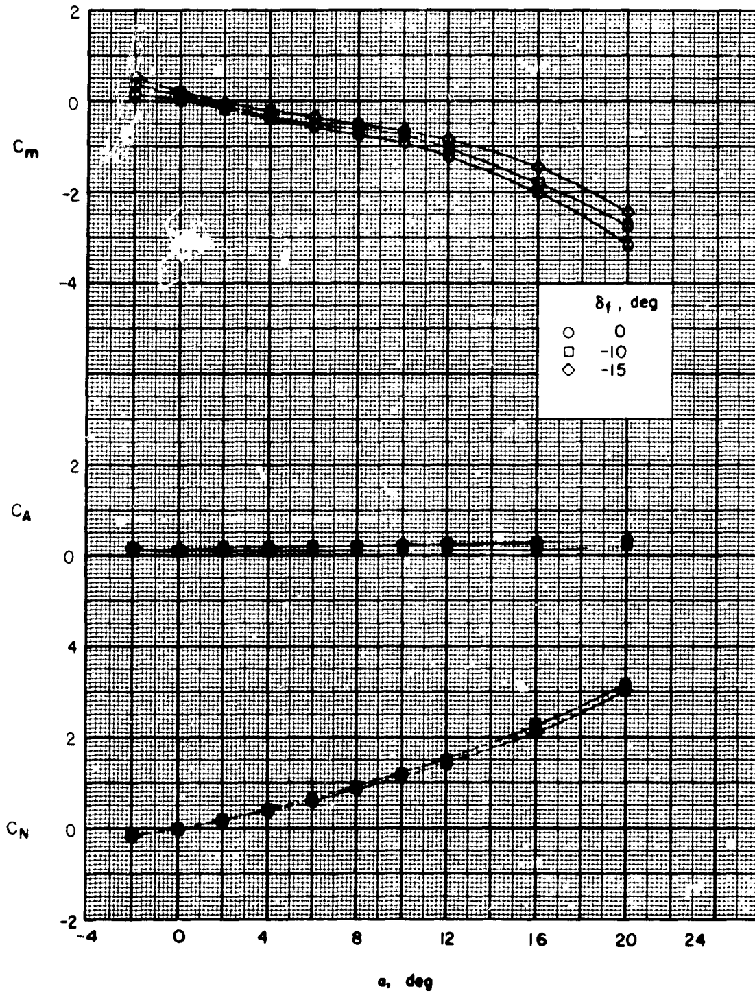
(a) Body axis.
