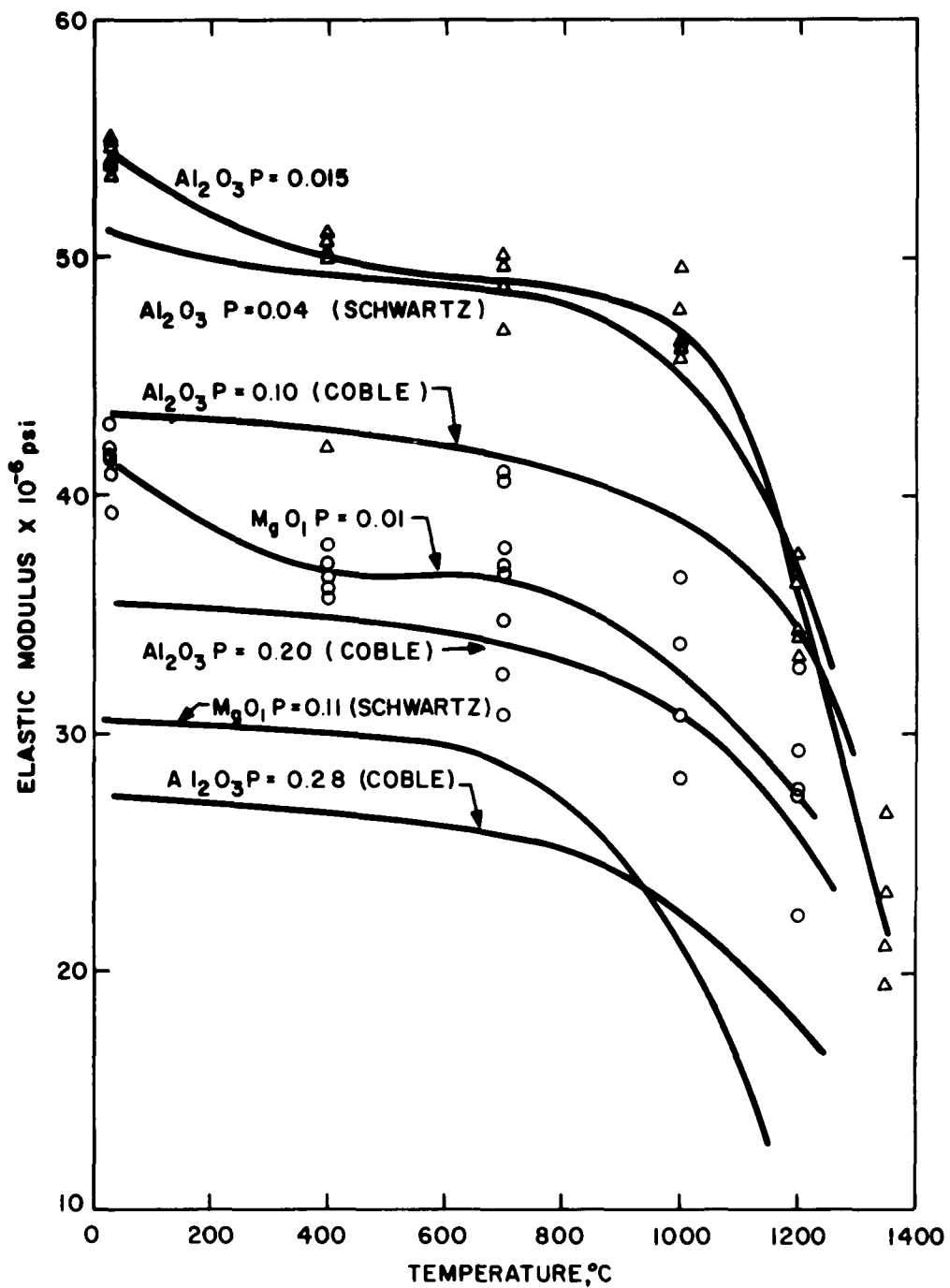
Figure 5. MODULUS OF ELASTICITY VERSUS TEMPERATURE 65-1946
