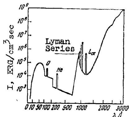
Fig. 2. Supposed energy distribution in the ultraviolet and X-ray spectrum of the sun.
