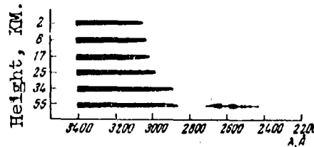
Fig. 1. Spectrograms obtained during flight of rocket (Kondrat'yev, 1954).
