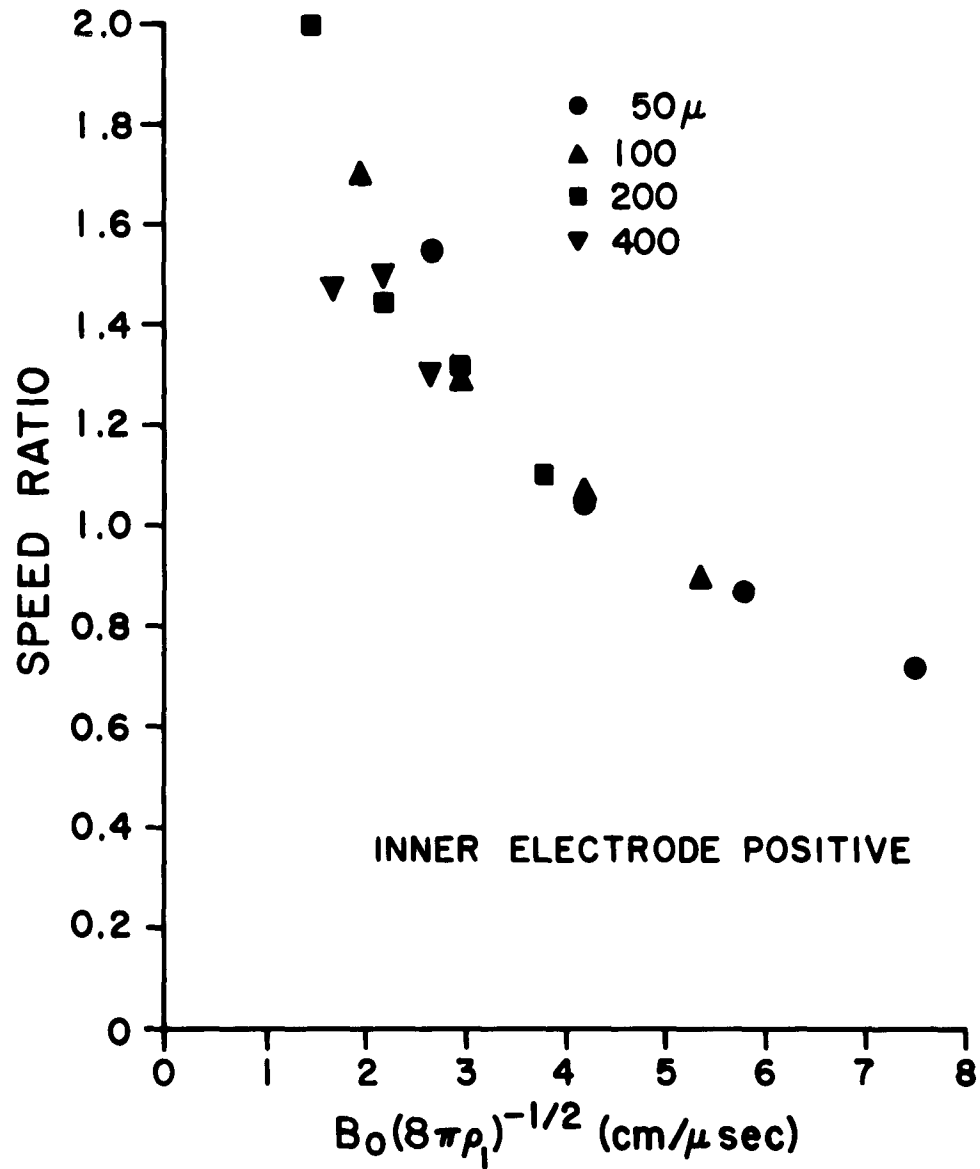
Fig. 7 Ratio of the speed of the current sheet observed by Keck to the speed u_s = B_0(8\pi\rho_1)^{-1/2} plotted against the latter speed. The points are coded according to the gas pressure (in microns) in the tube before the discharge.
