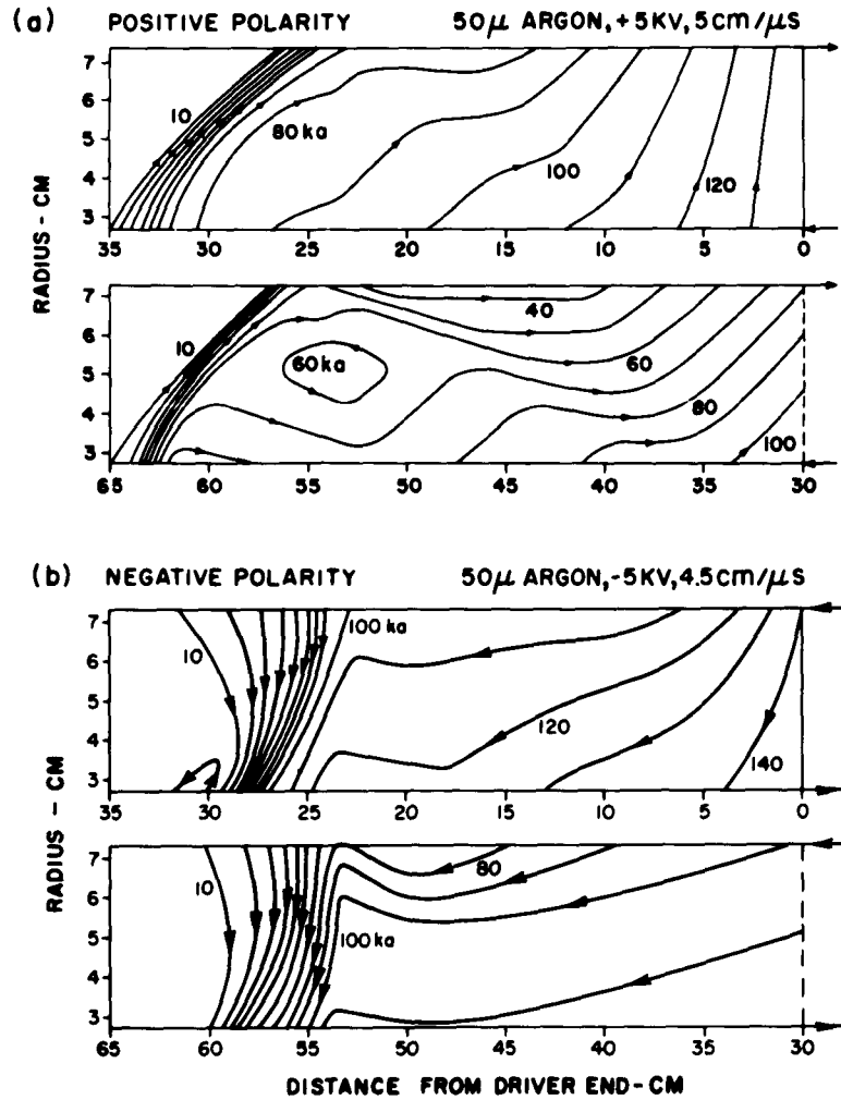
Fig. 4 Contour plots showing current distribution in the MAST for positive and negative center electrode. Note that the axial scale of the figure has been compressed by a factor of 2.
