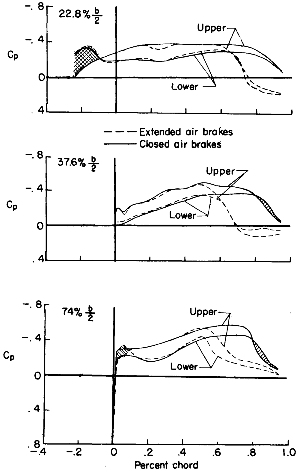
(b) \alpha = 0^\circ ; M = 1.03 . Concluded.
