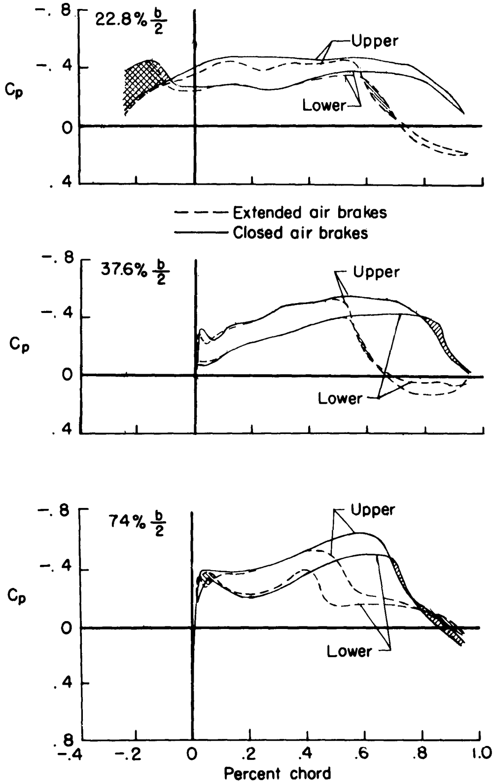
(b) \alpha = 0^\circ ; M = 0.98 . Continued.
