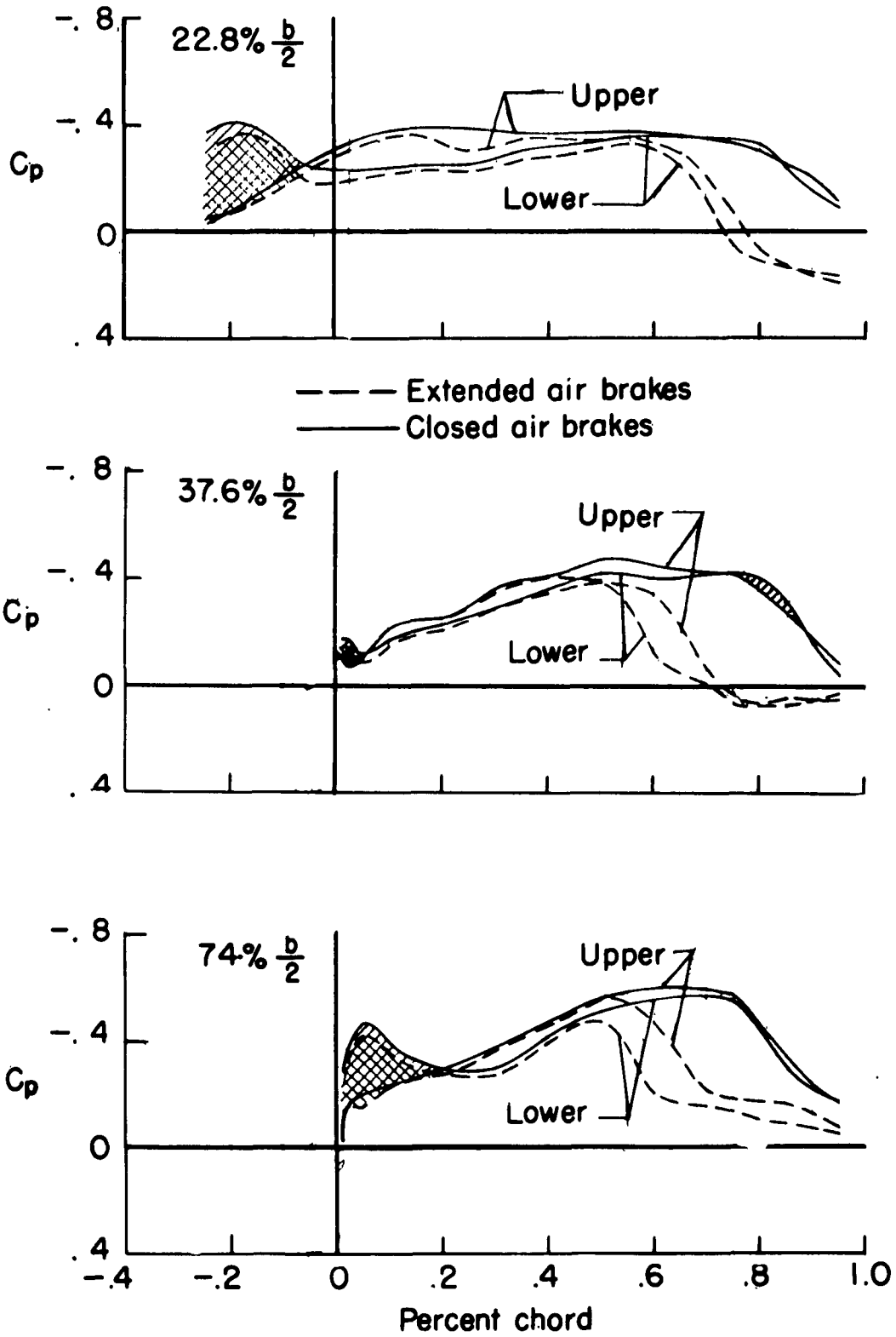
(a) \alpha = -2^\circ ; M = 1.03 . Concluded.
