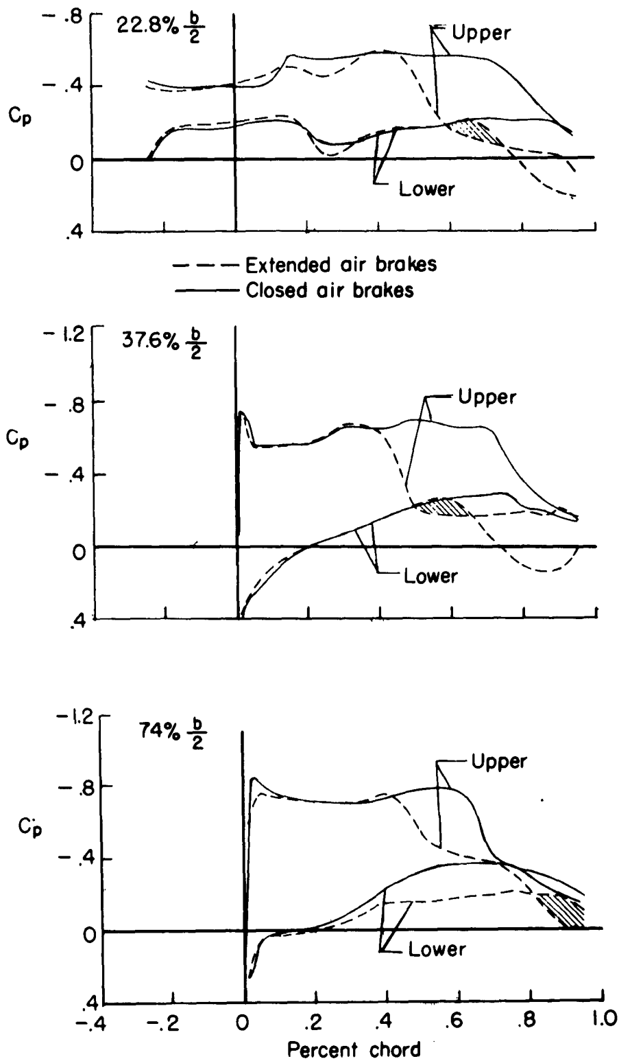
(c) \alpha = 4^\circ ; M = 0.98 . Continued.
