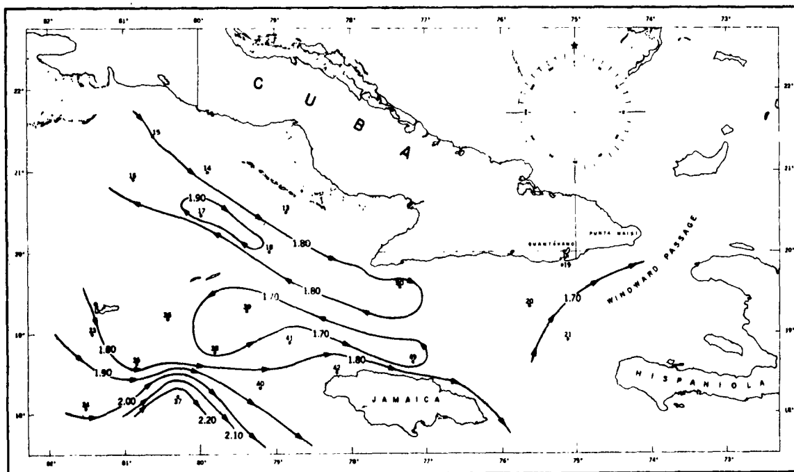
Fig. 1. Current pattern at surface determined from dynamic topography relative to 1,200-meter level
