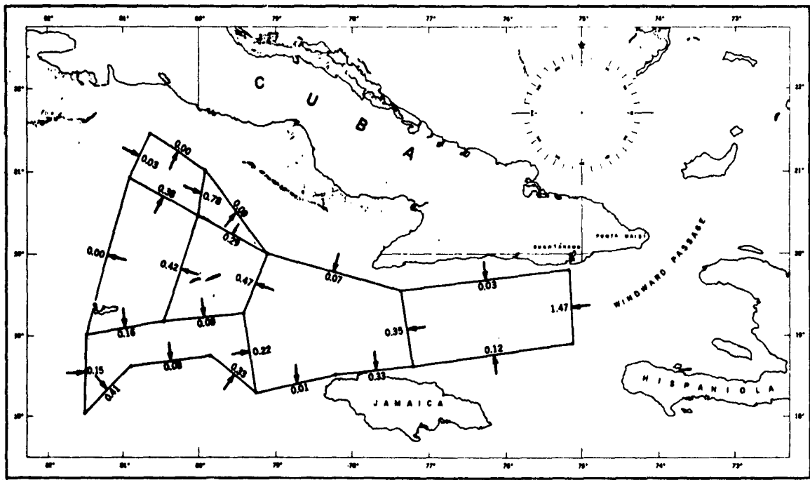
Fig. 10. Current speeds (knots) calculated from volume transport through cross sections of 920 meters average depth
