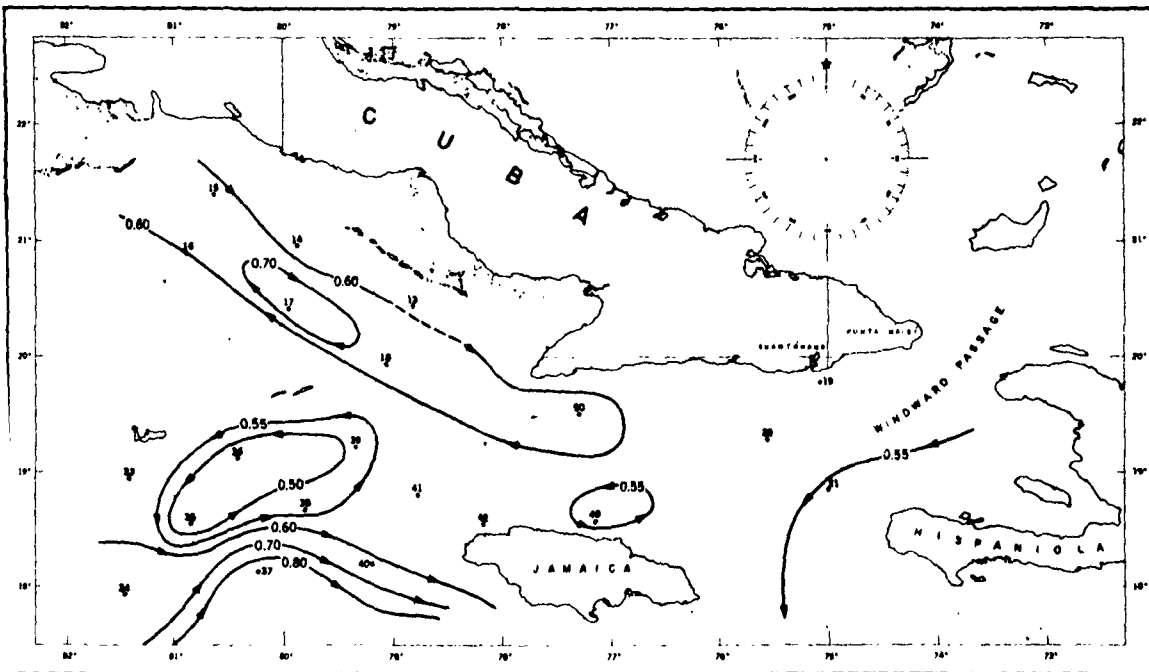
Fig. 3. Current pattern at 300 meters determined from dynamic topography relative to 1,200-meter level
