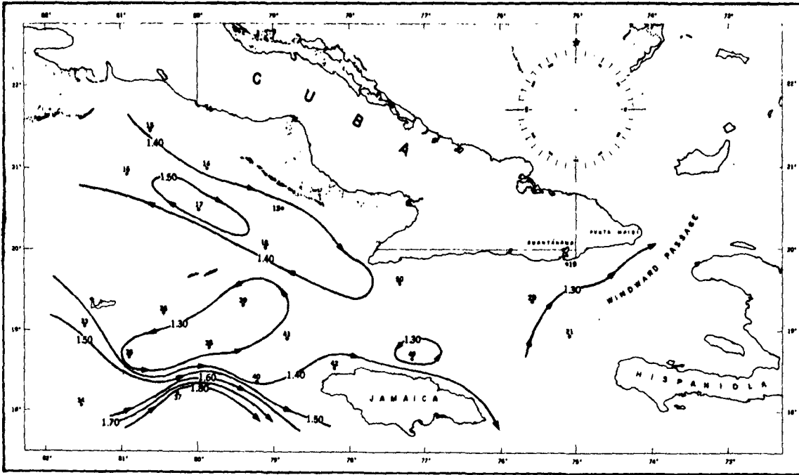
Fig. 2. Current pattern at 100 meters determined from dynamic topography relative to 1,200-meter level
