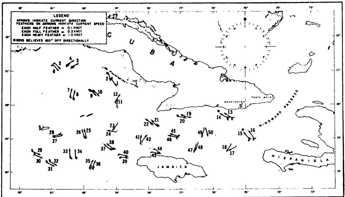
Fig. 6. Surface currents USS PURSUIT GEK observations 14-28 March 1953
