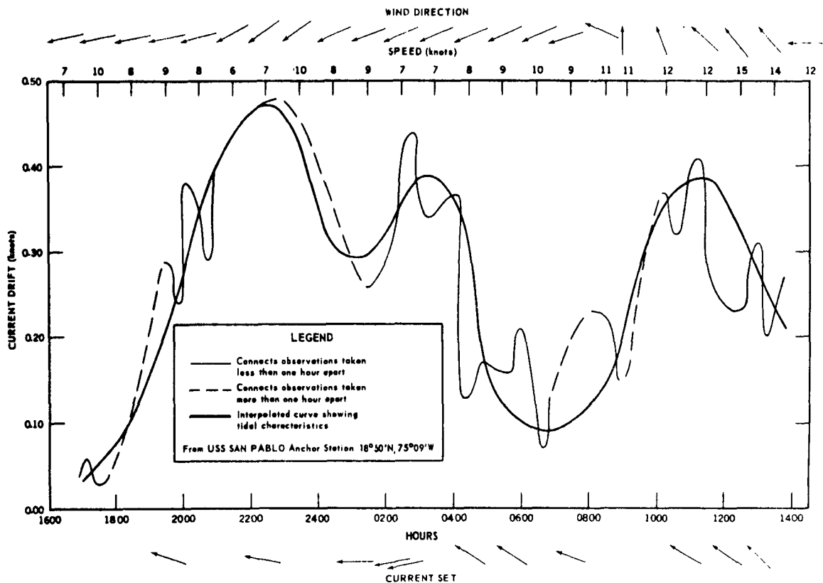
Fig. 14. Surface current measurements exhibiting tidal characteristics
