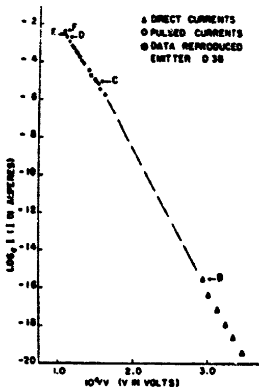
Fig. 3. Current-voltage relationship for combined direct current and pulsed operation of emitter O-38. Data at (B), (C), (D), (E), and (F), correspond to the data at the same letters in Fig. 2. Space-charge effects were observed at currents above (C); anomalies in the normal emission preceding electrical breakdown were observed from (D) to (F).
