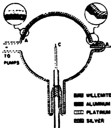
FIG. 1. Experimental field emission tube. ( C ), field cathode; ( A ), aluminum-lacquer-willemite anode.
