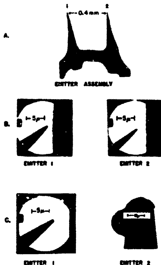
FIG. 5. (A), optical micrograph of twin emitter assembly showing emitter No. 1 and emitter No. 2 as marked. (B) electron micrographs before use. (C) electron micrographs after use.
