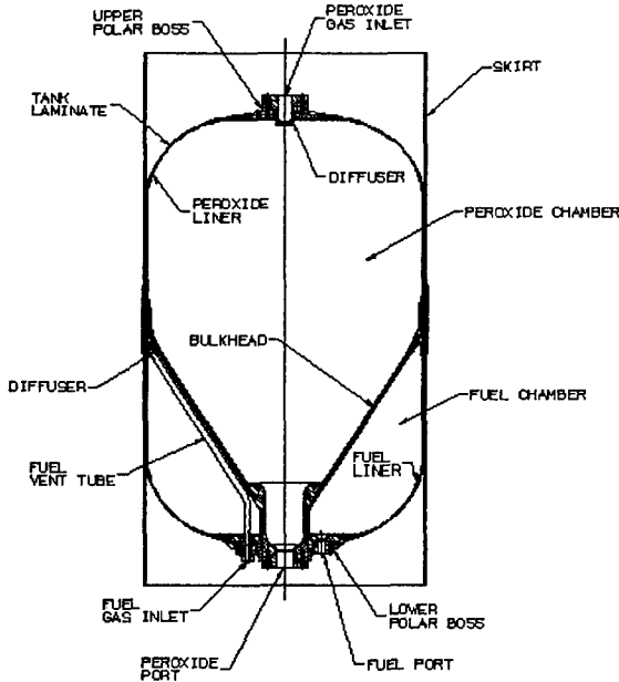
Fig. 3. Subscale integral structure configuration.
