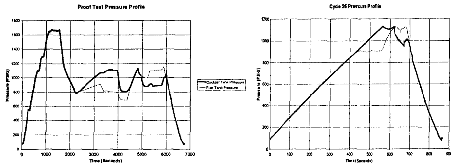
Fig. 24. Test pressure cycling to MEOP.
