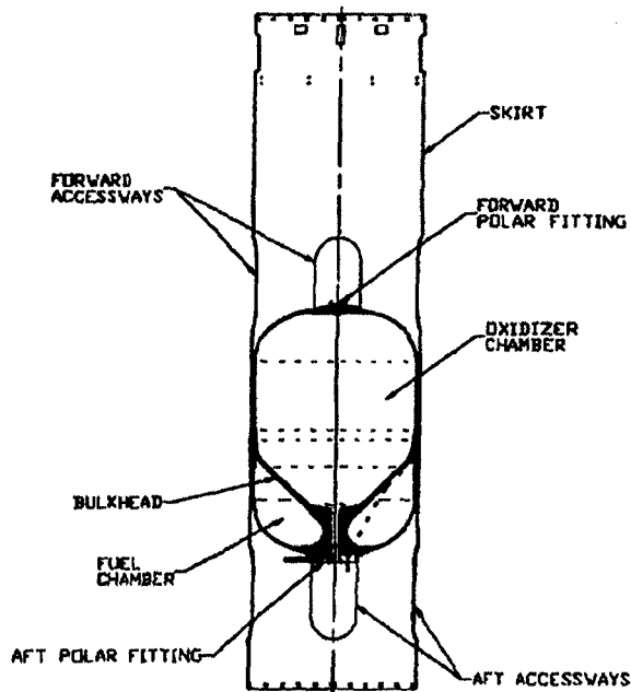
Fig. 4. Flight unit USFE integral structure configuration.
