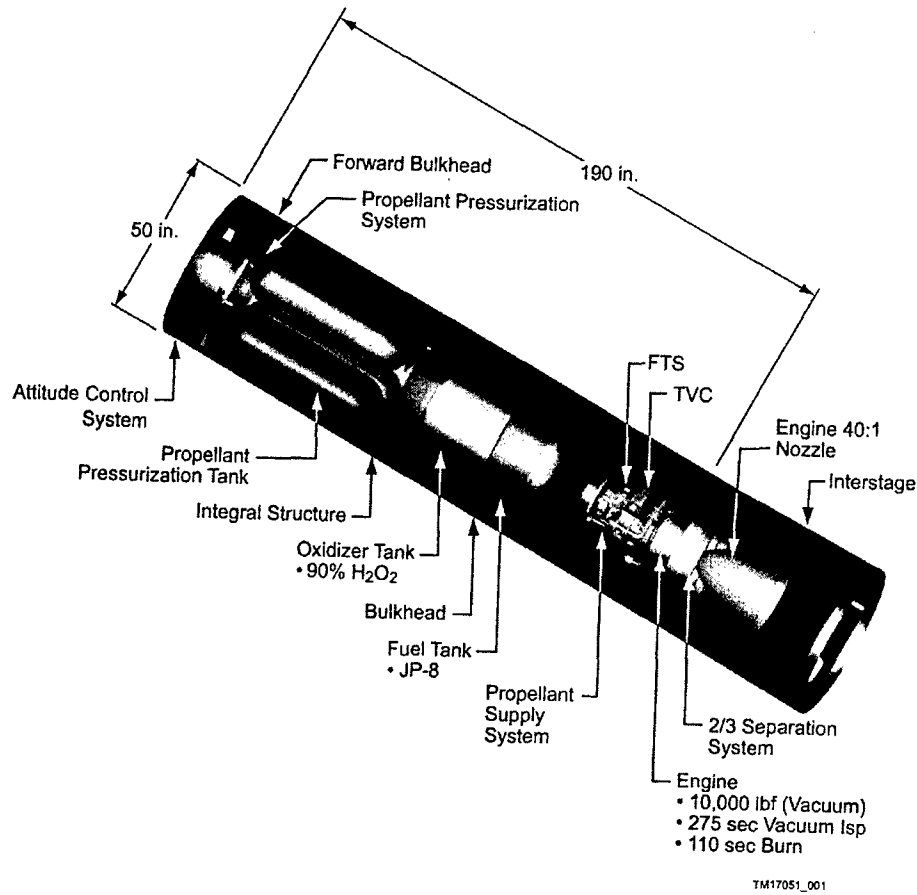
Fig. 2. USFE Stage with attached OSP interstage.
