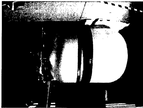
Fig. 14. Oxidizer liner assembly.
