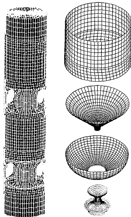
Fig. 5. FEA model of the structure.
