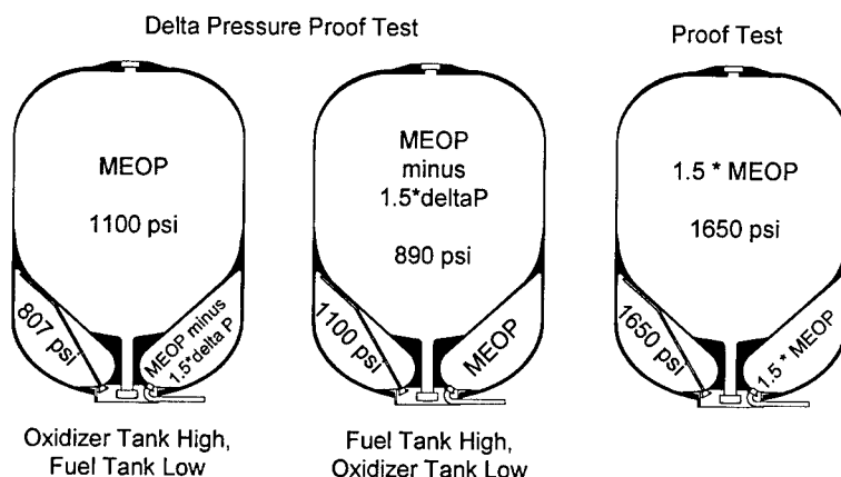
Fig. 23. Integral structure pressure testing (skirt no shown).
