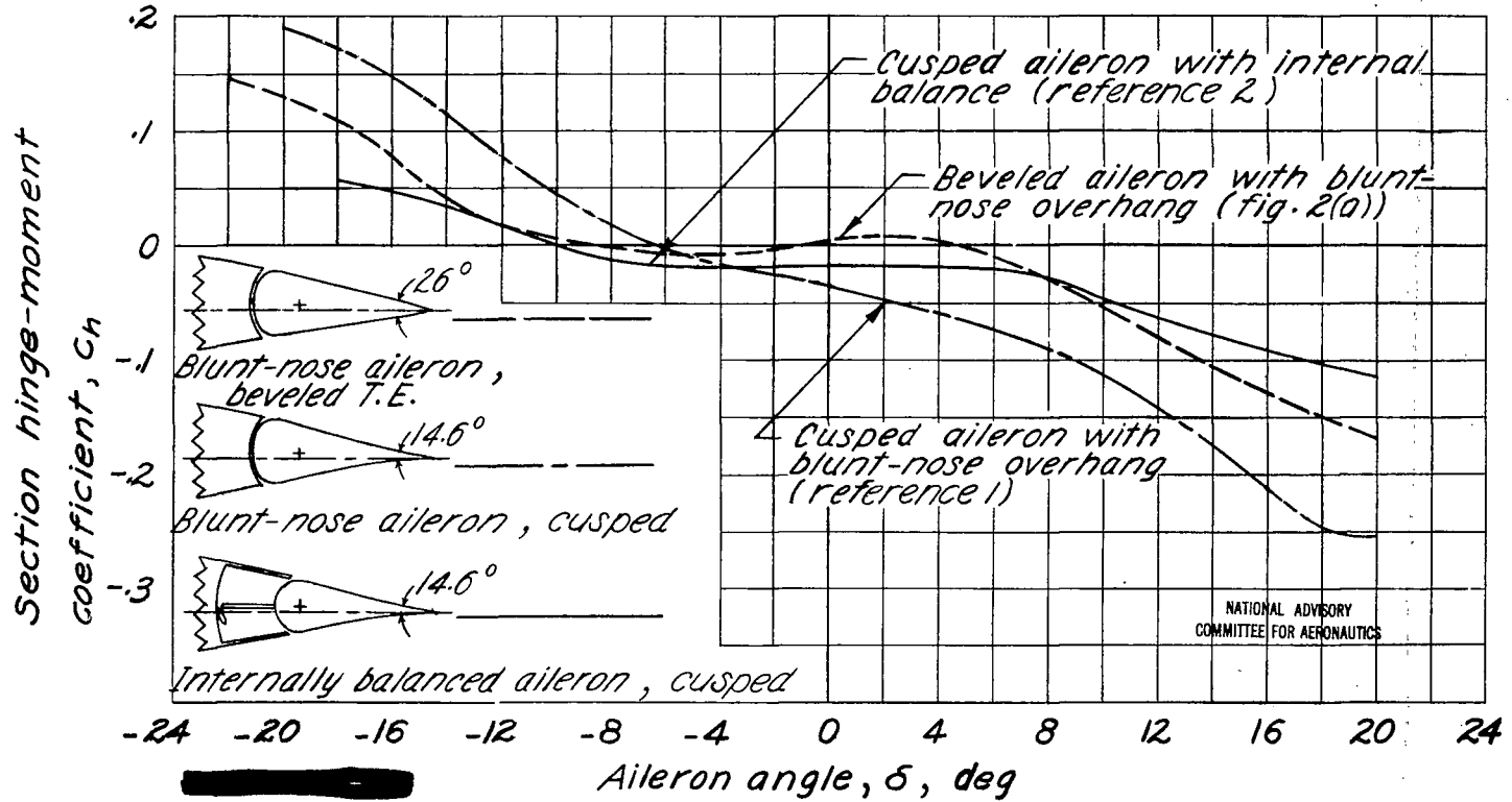
Figure 15.—Variation of section hinge-moment coefficient with aileron angle. \alpha_o = 0^\circ . All ailerons sealed.
