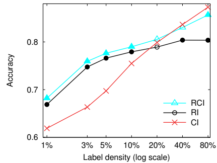
Figure 1: Accuracy for “Gene” using Naive Bayes and SSL-ONCE (see Section 5). Within a column, a circle or triangle that is filled in indicates a result that was significantly different (better or worse) than that of CI.
