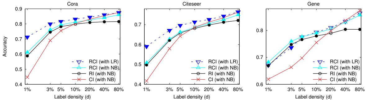
Figure 2: Accuracy vs. label density. Solid lines show results with NB; for these, filled (not hollow) symbols indicate sig. differences vs. CI. Dashed lines show RCI+LR for comparison; for these, filled symbols mean sig. differences vs. RCI+NB. These results (as with all others, unless otherwise stated) use SSL-ONCE and, where needed, ICA for inference.
