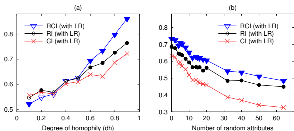
Figure 3: Synthetic data results, using LR and 5% label density. Filled symbols indicate sig. differences vs. CI.
