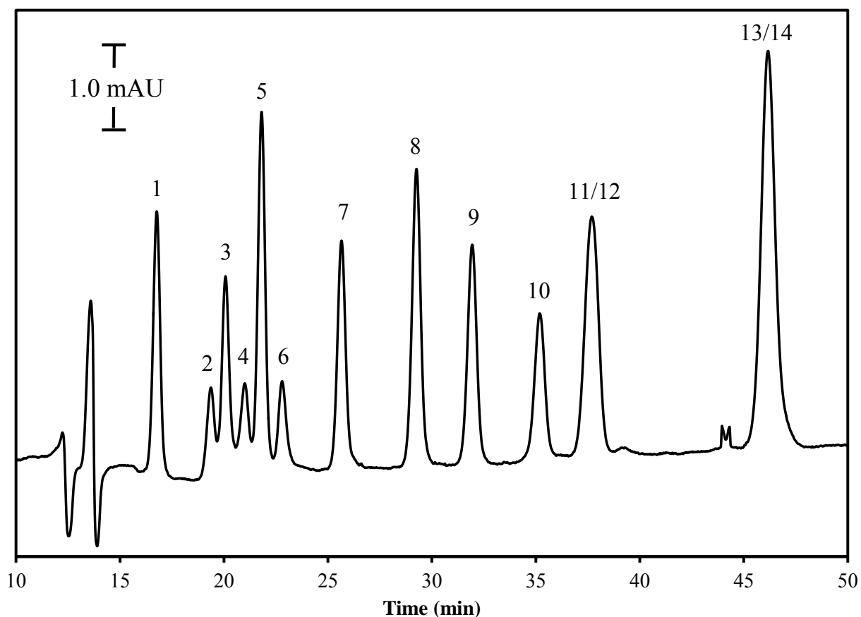
Figure 2. Representative electropherogram for a mixture of 14 nitroaromatics, nitramines and their degradation products. Sample concentration was 5 \mu\text{g mL}^{-1} for all analytes. See Table 1 for compound listing.
