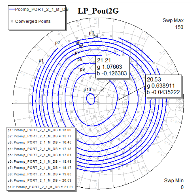
Figure 2. A 2-GHz load-pull simulation of output power (Pcomp-6 x 65 \mu m PHEMT).
