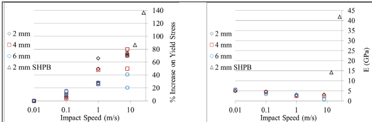
Figure 4. Comparison of the yield strength (left) and elastic modulus (right) of CMF at various speeds.
