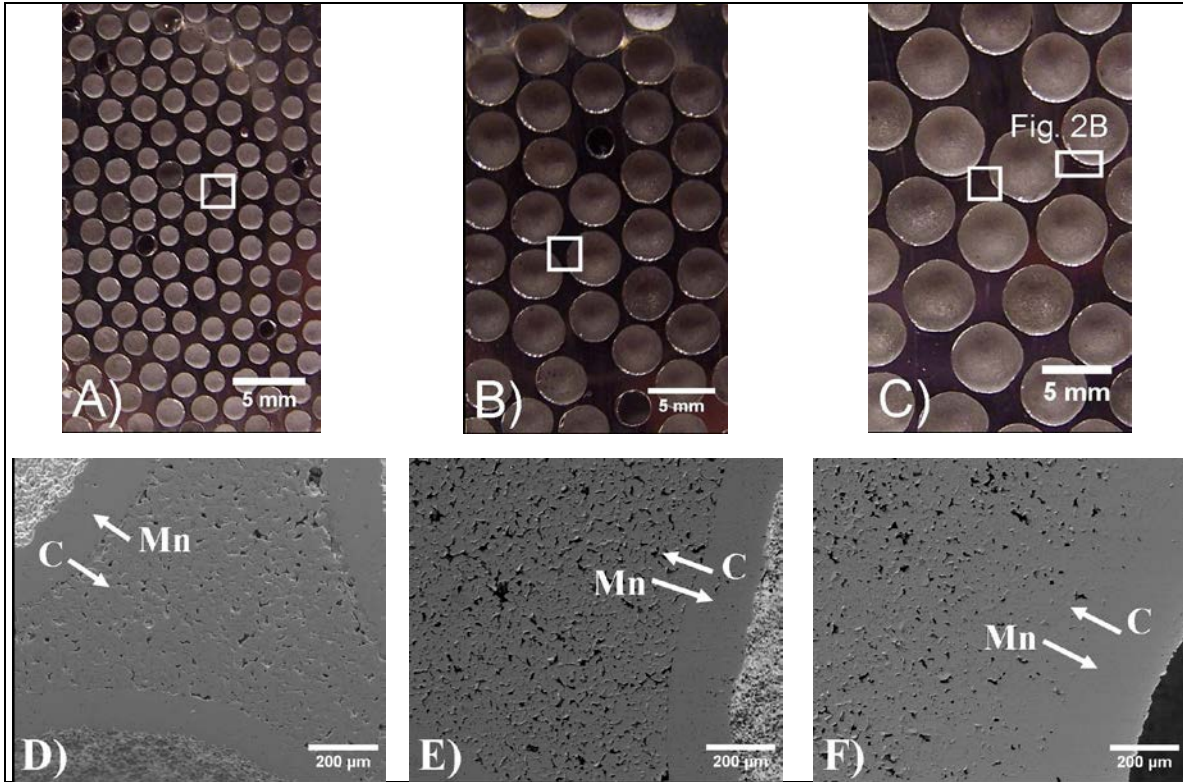
Figure 1. (A), (B) and (C) Digital images of the composite foam with 2.2-, 4- and 5.2-mm sphere diameters, (D), (E) and (F) corresponding SEM images of the area highlighted with the box in each image respectively.
