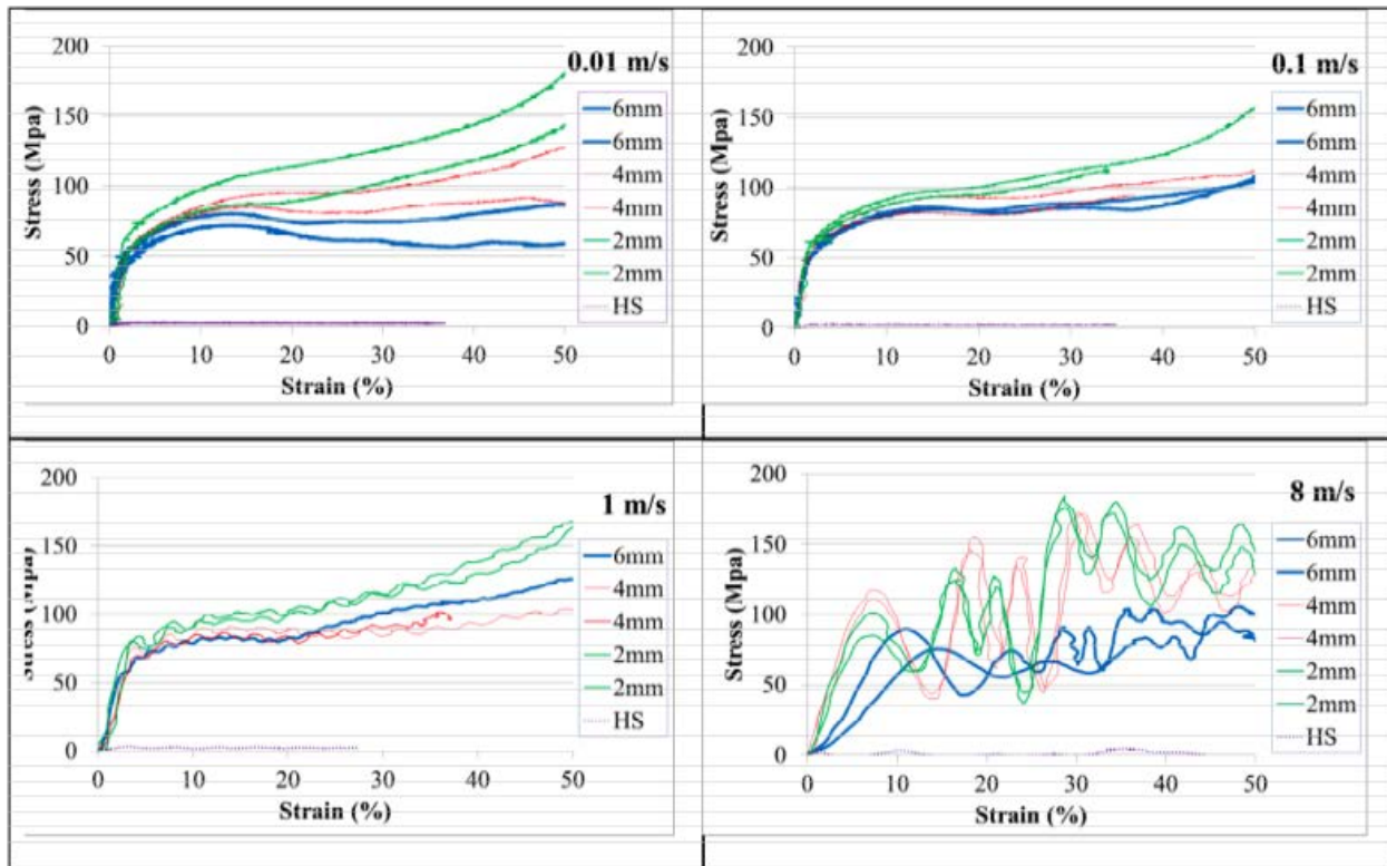
Figure 3. Stress-strain curve for samples with various sphere sizes under various loading speeds.
