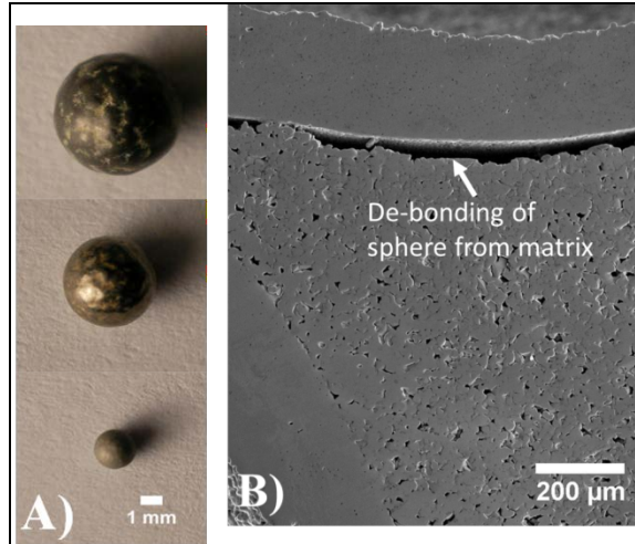
Figure 2. Surface features of hollow spheres (A), and the presence of limited debonding at the interface (B).
