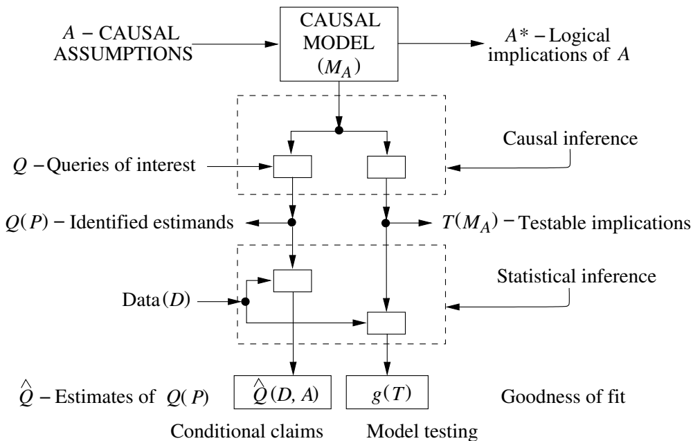
Figure 1: SEM methodology depicted as the an inference engine converting assumptions ( A ), queries ( Q ), and data ( D ) into logical implications ( A^* ) Conditional claims ( C ) and data-fitness indices ( g(T) ).
