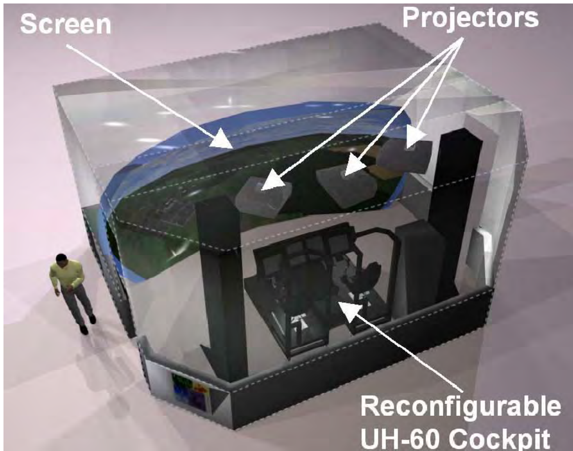
Figure 7. UH-60M BHIVE 1 configuration.
