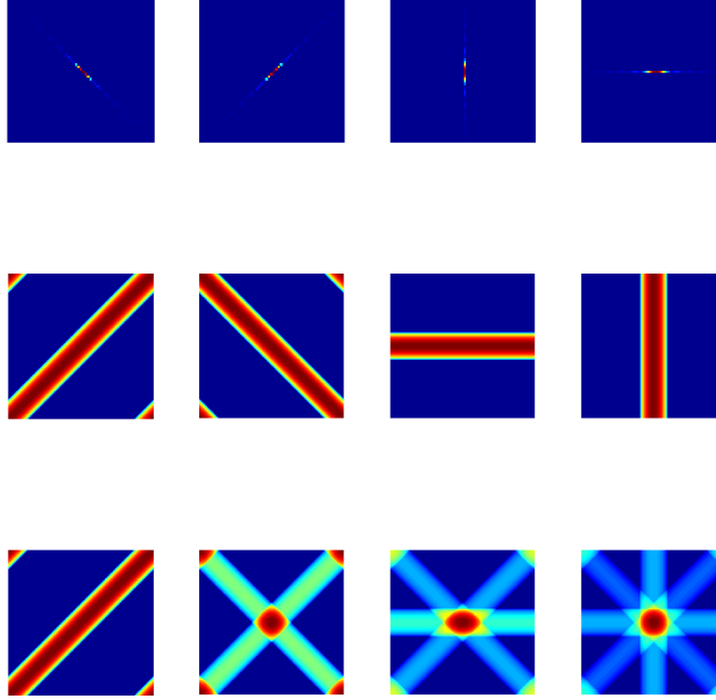
Fig. 7. From the object in Fig. 5, slices of the 2-D spatial-frequency domain for different look angles (top row) are inverse Fourier transformed (middle row), and added together to form an image (bottom row).
