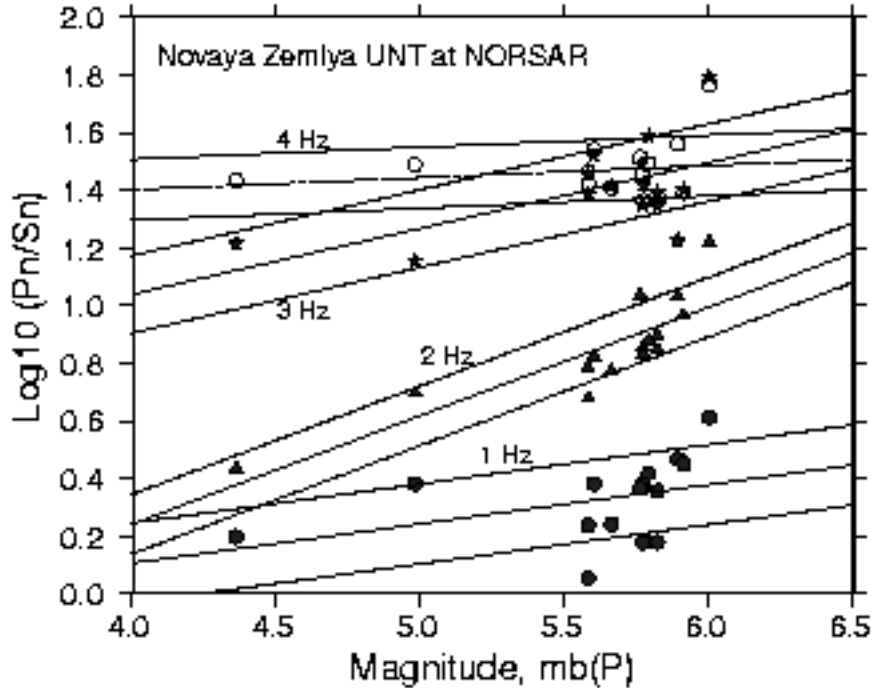
Fig. 2 \text{Log}_{10}(Pn/Sn) spectral ratios of each event are plotted against magnitudes for frequencies 1 to 4 Hz. The Pn/Sn ratios in the frequency bands 1–4 Hz indicates a weak magnitude dependence of Pn/Sn ratios. The slope (thick line) and the standard deviation ( \pm 2\sigma ) of the regression (dotted lines) are plotted for reference.
