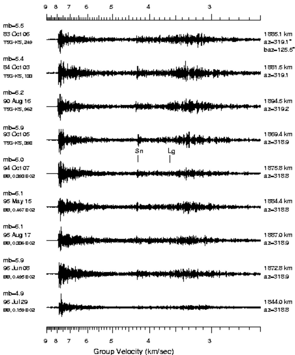
Fig. 3 Vertical component records at BRVK in northern Kazakhstan from underground nuclear tests from Lop Nor. Records are plotted with group velocity in km/sec and magnitude, m_b(P) , of each event is indicated at the beginning of each trace. BB indicate broadband signals from the new instrument (STS-2 sensors), while TSG-KS indicate signals recorded by STsR-TSG KS system with SKM-3 sensor.
