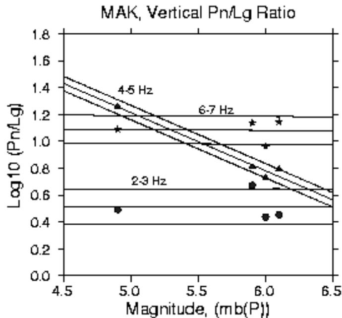
Fig. 5 (upper panel) Vertical records from four Chinese underground nuclear tests at Lop Nor recorded at MAK (Makanchi). Event id, magnitude and zero-to-peak amplitude in micrometer/sec is indicated at the beginning of each trace. Notice the considerable variation of Lg waves excitation from each event. (lower panel) \text{Log}_{10}(\text{Pn/Lg}) spectral ratios at three frequency bands are plotted against magnitude. Notice a negative slope at 4-5 Hz band, which is due to strong P wave spectral peak at this frequency on signal from the event on July 29, 1996.
