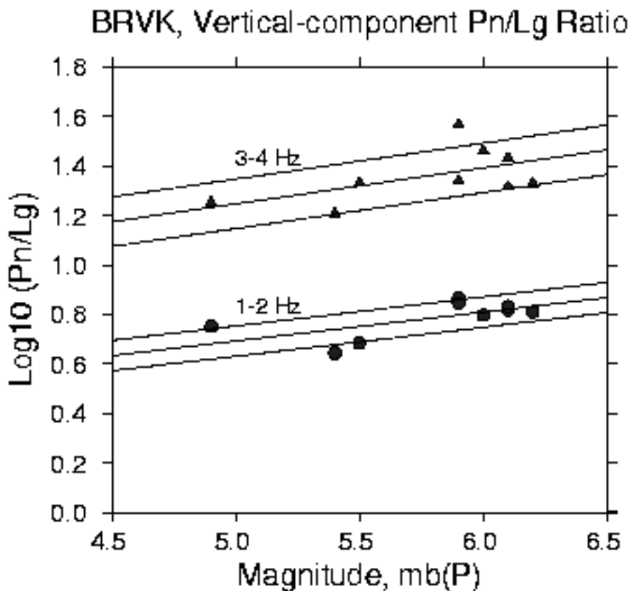
Fig. 4 \text{Log}_{10}(Pn/Lg) spectral ratios of each event are plotted against magnitudes for frequency band 1-2 Hz and 3-4 Hz. Pn/Lg ratios in the frequency bands 1-4 Hz indicate a very weak magnitude dependence of Pn/Lg ratios. The slope (thick line) and the standard deviation ( \pm 2\sigma ) of the regression (dotted lines) are plotted.
