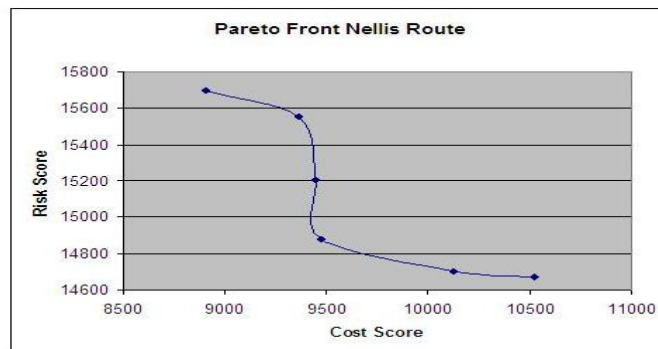
Figure 6 Risk vs. Cost Pareto Front
