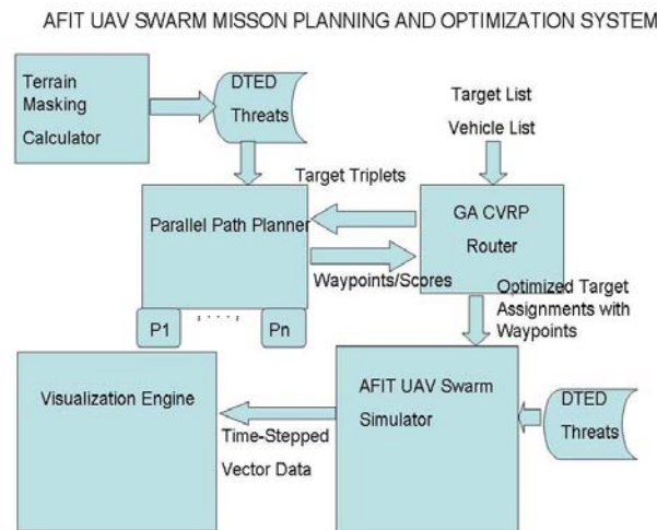
Figure 4 System Data Flow Design
