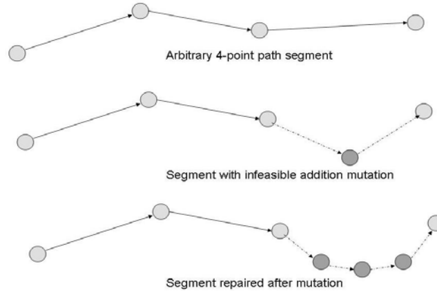
Figure 2 Mutate Add Operation on 4-point Path Segment.
