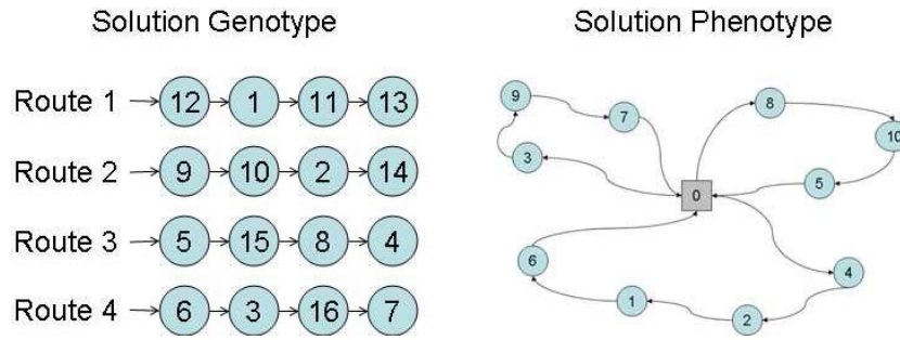
Figure 3. GVR chromosome structure for the VRP
