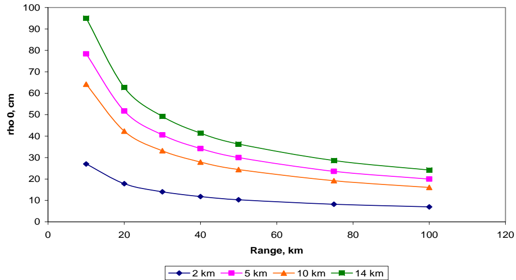
Figure A-7. Variation of \rho_0
