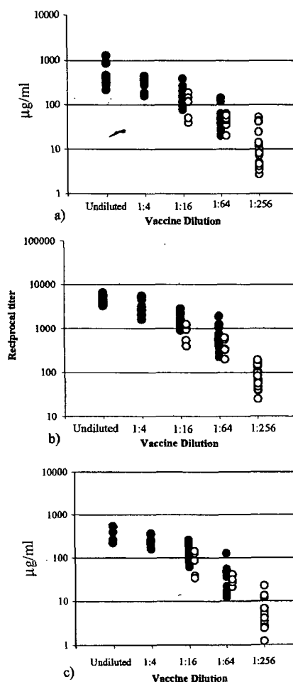
Fig. 2. Relationship between survival in AVA-vaccinated rabbits (Lot FAV 032) after aerosol challenge with B. anthracis spores and antibody response. The vaccine dilution is plotted against (a) the anti-PA IgG concentration ( \mu\text{g/ml} ) at 6 weeks; (b) the reciprocal TNA titer at 6 weeks; and (c) the anti-PA IgG concentration ( \mu\text{g/ml} ) at 9–10 weeks. Individual animals surviving (●) or dying (○) after challenge are indicated.
