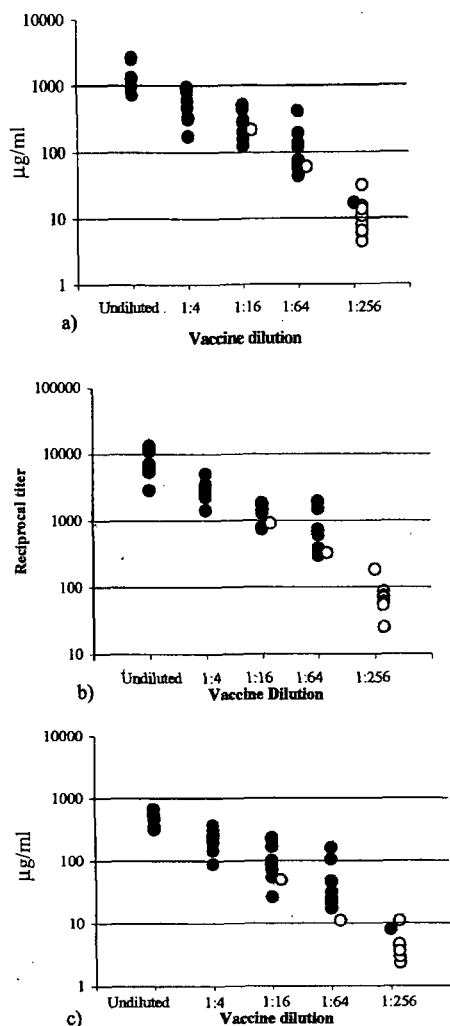
Fig. 1. Relationship between survival in AVA-vaccinated rabbits (Lot FAV 008) after aerosol challenge with B. anthracis spores and antibody response. The vaccine dilution is plotted against (a) the anti-PA IgG concentration ( \mu\text{g/ml} ) at 6 weeks; (b) the reciprocal TNA titer at 6 weeks; and (c) the anti-PA IgG concentration ( \mu\text{g/ml} ) at 9–10 weeks. Individual animals surviving (●) or dying (○) after challenge are indicated.
