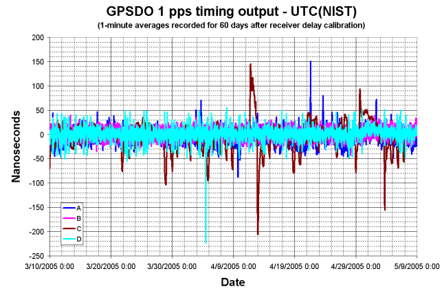
Figure 2. Phase plot of GPSDO 1 pps – UTC(NIST) using known antenna coordinates.
