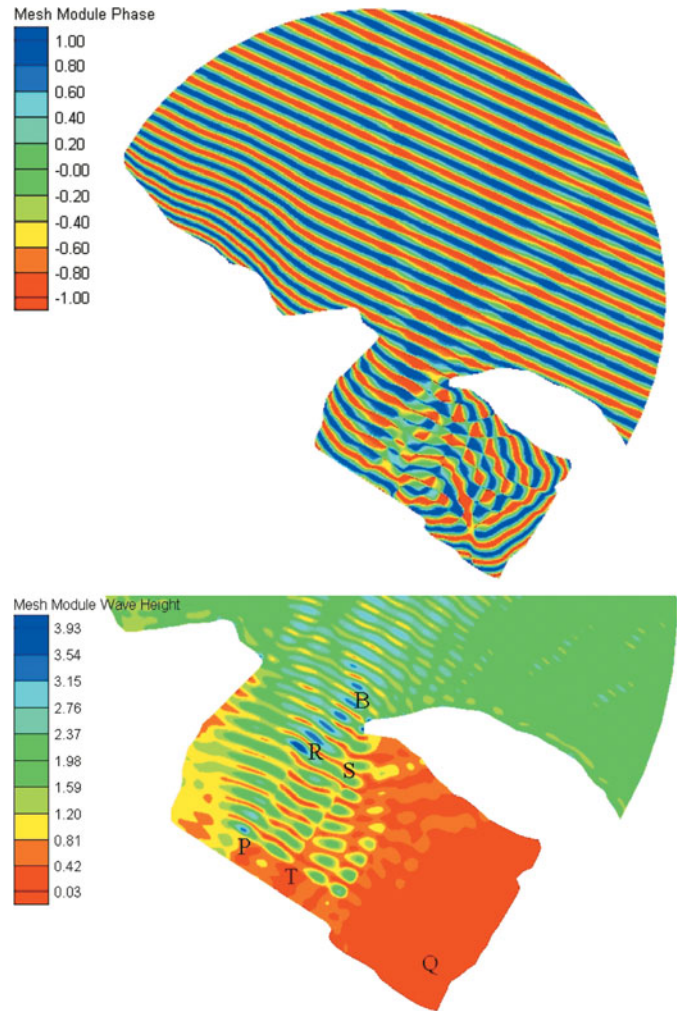
Fig. 14. Modelled phases and wave heights (metres) in Douglas Harbor, with docks.
