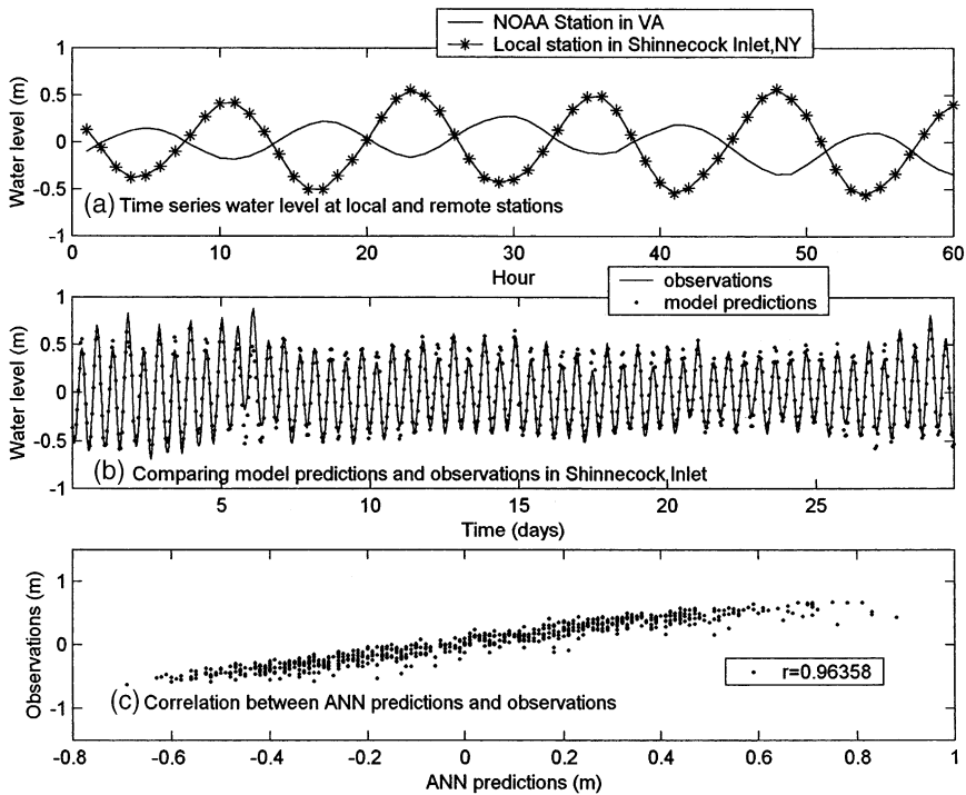
Fig. 14. Model test using water level inputs from a remote NOAA station located 466 km away in the coast of Lewisetta, Virginia.
