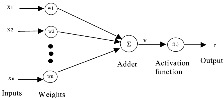
Fig. 3. One neuron structure.
