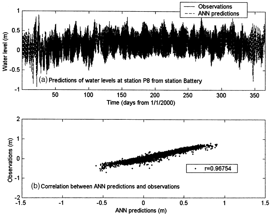
Fig. 9. Comparison of water levels between model predictions and observations at station P8 Fire Island Inlet for year 2000. The distance between input NOAA station at Battery and the local station is about 90 km.
