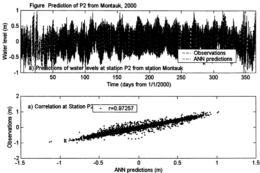
Fig. 8. Comparison of water levels between model predictions and observations at station P2 of Shinnecock Inlet for year 2000. The distance between input NOAA station at Montauk and the inlet is about 60 km.
