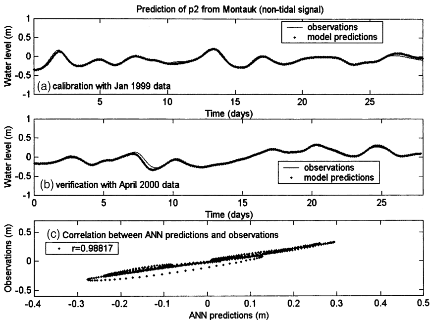
Fig. 10. Model test for non-tidal water level predictions at station P2. The distance between input NOAA station at Montauk and the inlet is about 60 km.
