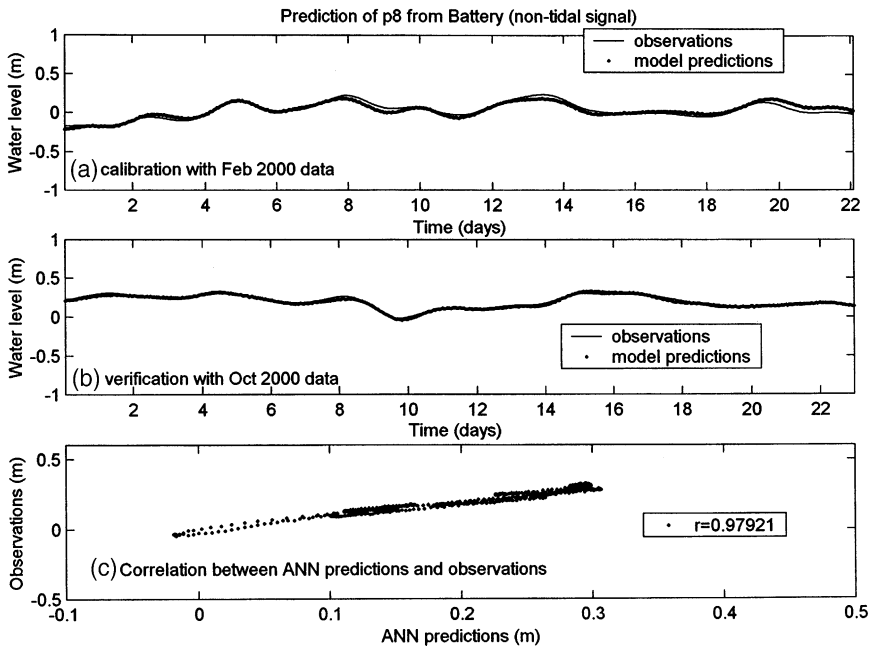
Fig. 11. Model test for non-tidal water level predictions at station P8. The distance between input NOAA station at Battery and the local station is about 90 km.
