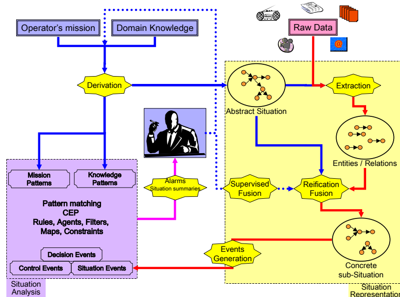
Figure 1: Information Flow
