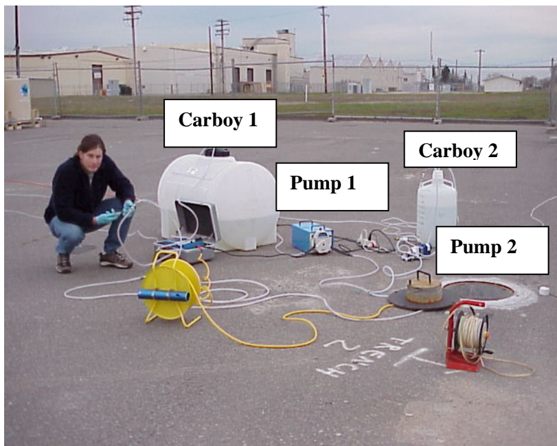
Figure 3. Typical Field Setup for Push-Pull Tests.
