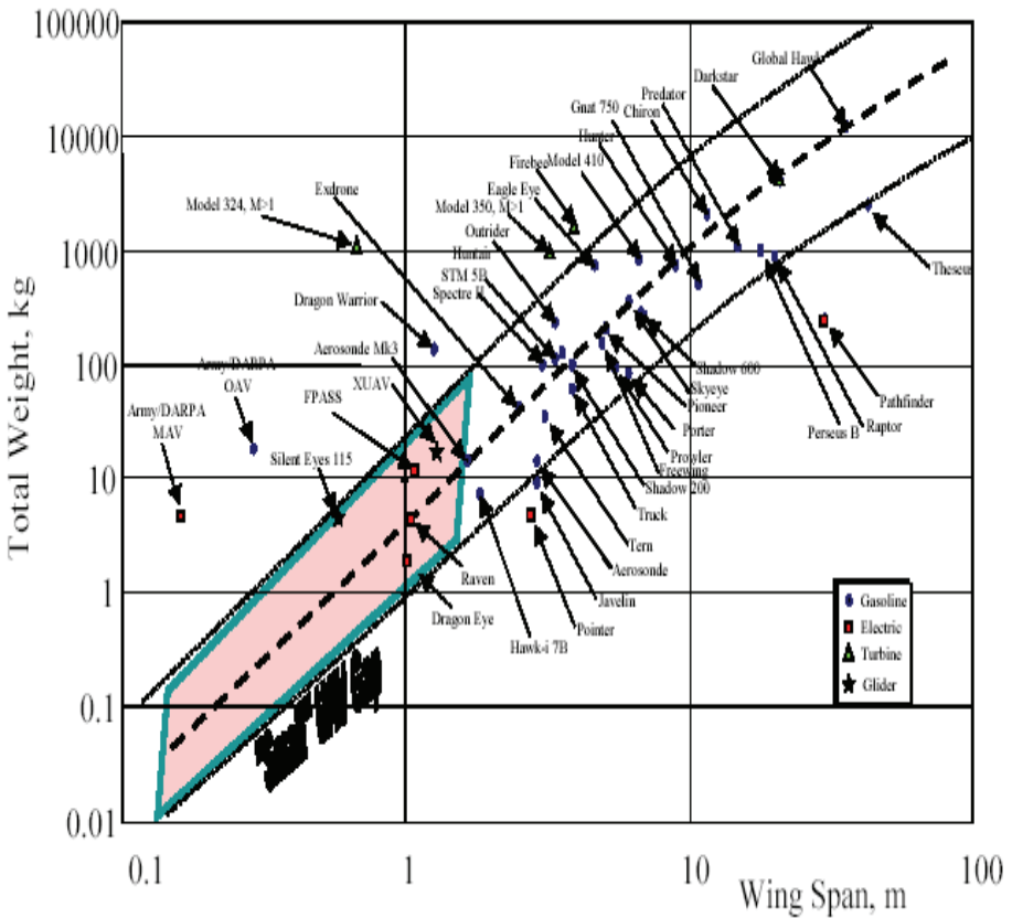
Figure 7.1 UAV Weight vs. Wing Span 17
