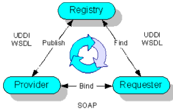
Fig. 3. The W3C Model of the SOA Concept
