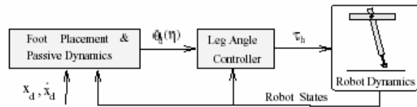
Figure 2: Velocity controller
