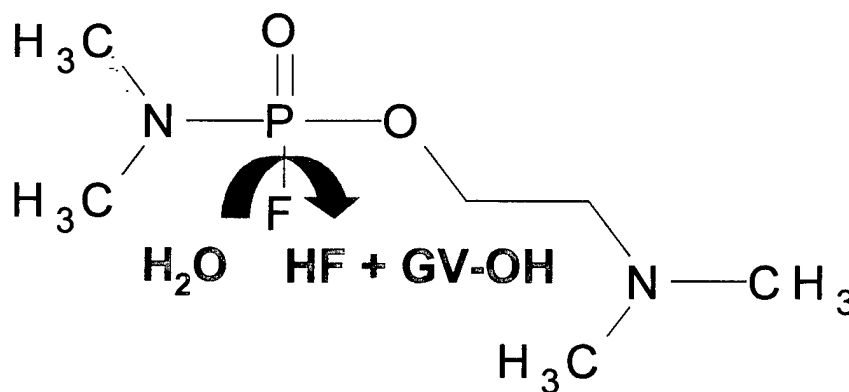
Figure 2. Reaction Scheme for the Hydrolytic Defluorination of GV
