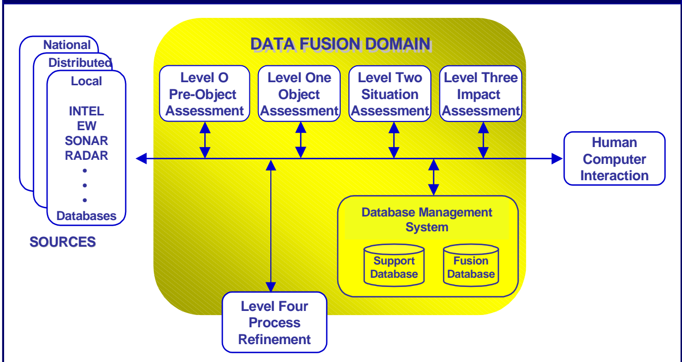
Figure 1: Top Level View of the JDL Data Fusion Process Model
