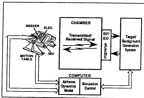
Figure 19. Generic HWIL Diagram
