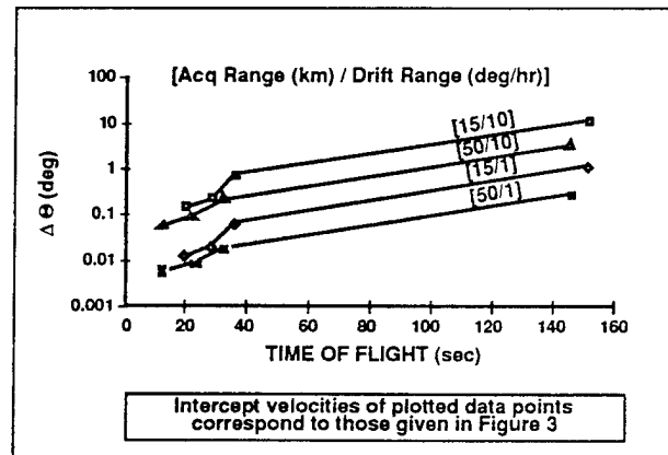
Figure 17. IMU Drift Rate Error Analysis
