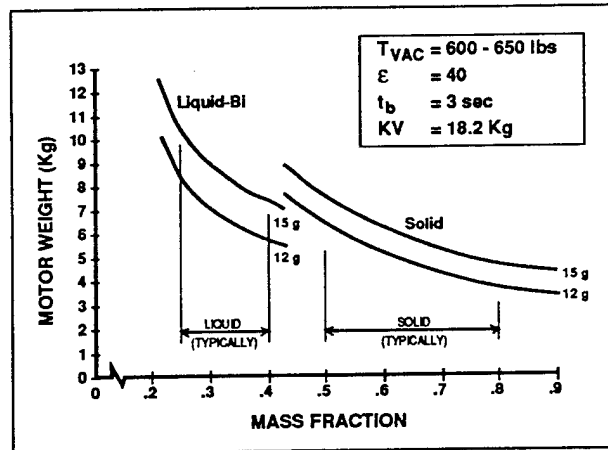
Figure 14. Typical Divert Propulsion System
