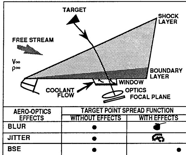
Figure 5. Aero-Optical Effects
