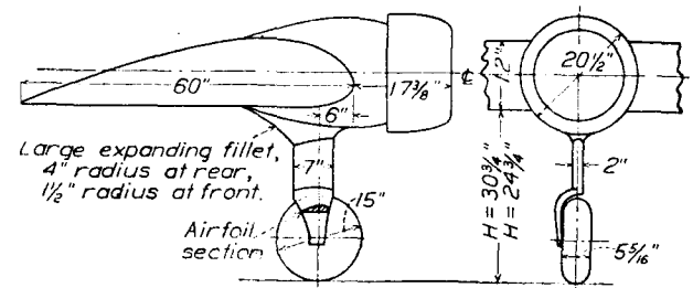
FIGURE 5.—Landing gear C.
