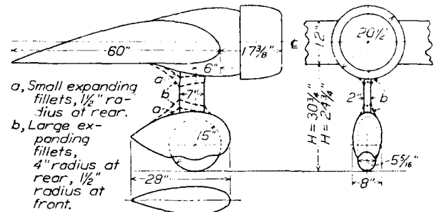
FIGURE 4.—Landing gear B.
