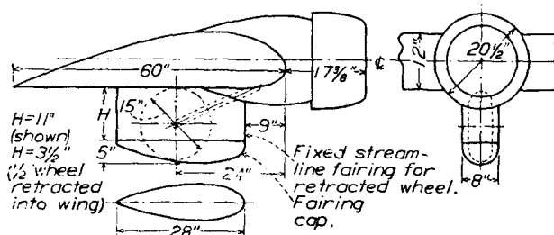
FIGURE 7.—Landing gear D retracted into streamline fairing.
