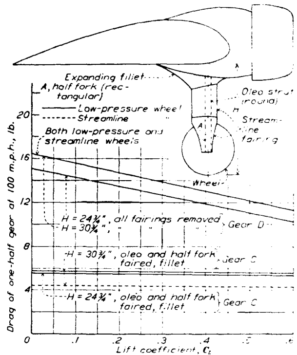
FIGURE 19.—Drag of landing gears C and D in presence of wing and nacelle
