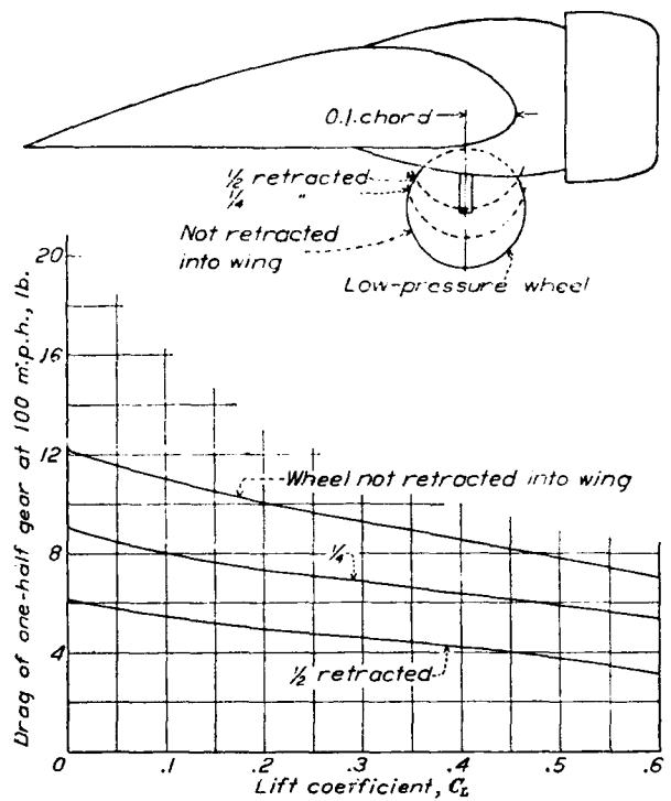
FIGURE 20.—Drag of landing gear D retracted vertically by various amounts into nacelle.
