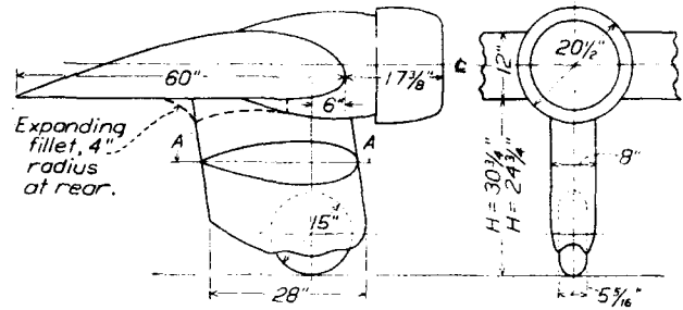
FIGURE 3.—Landing gear A.
