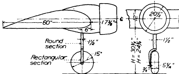
FIGURE 6.—Landing gear D.
