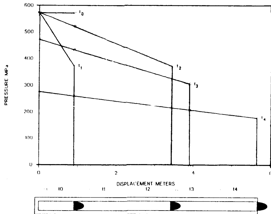
Figure 2. Pressure-Displacement, EE = 37 MJ.
