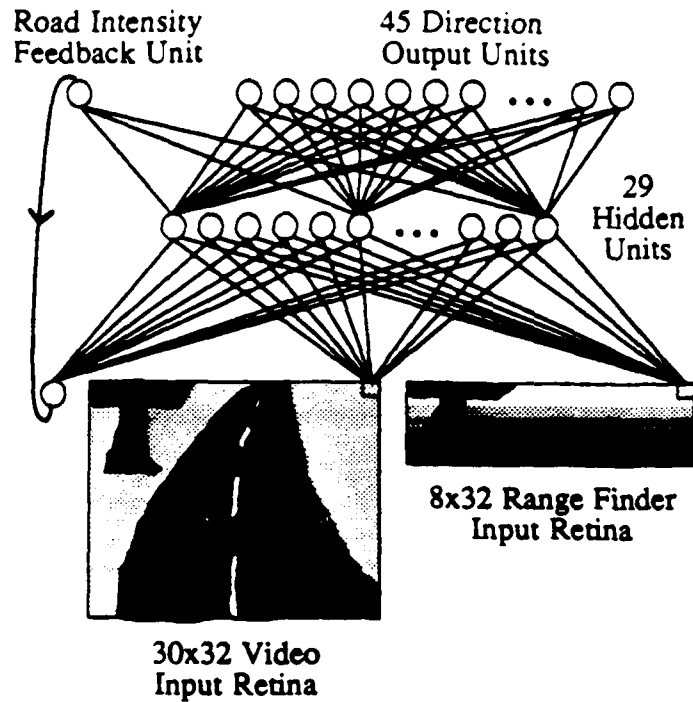
Figure 1: ALVINN Architecture
