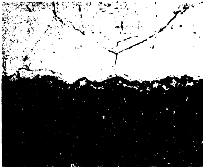
Figure 2. Microphotograph Shows Ductile Interface Alloy Formed When Copper Is Molten Welded To Steel.
