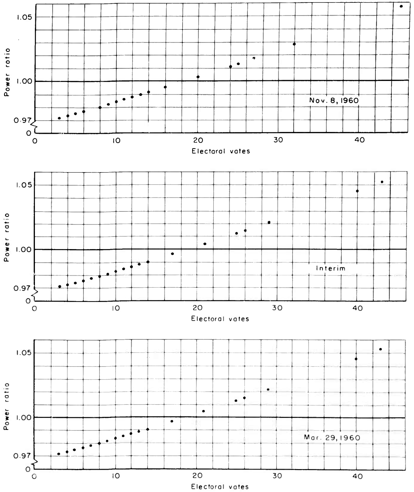
Fig. 1— Power ratio as a function of voting strength
