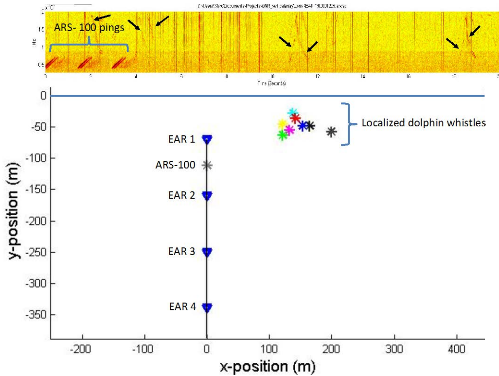
Figure 4 – Top panel: Spectrogram of a series of pings from the ARS-100 and concurrent dolphin whistles (arrows). Lower panel: localized positions of the pings and whistles relative to the array. The grey asterisk is the localization of the pings from the pinger. The dolphin whistles are plotted in color, with red being the most recent and gray the oldest in the sequence.
