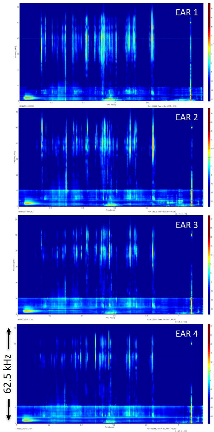
Figure 3 – Long-term spectral average of an odontocete encounter that occurred during the nighttime hours between August 8 th and 9 th recorded on the four EAR2s of the bottom-moored array. EAR #1 was closest to the surface and EAR #4 was closest to the bottom. The recorders were spaced 90 m apart.
