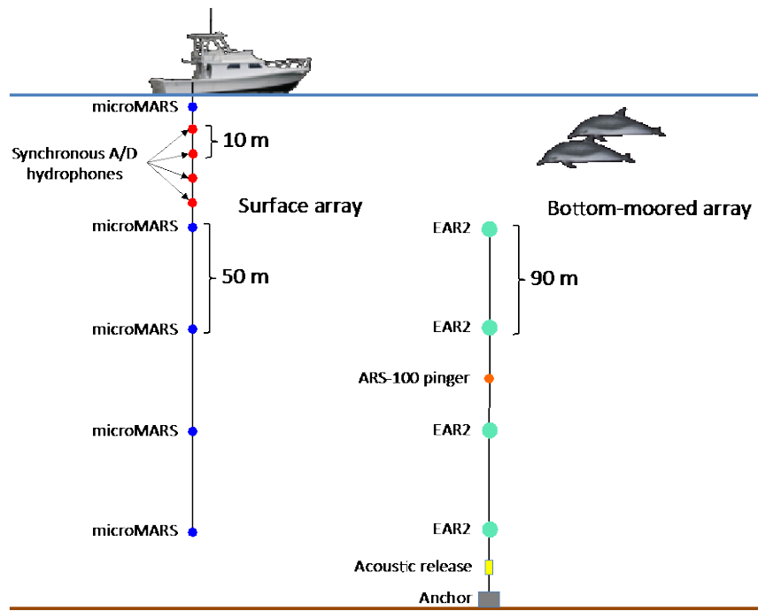
Figure 1 - Schematic of the surface array and bottom-moored array that will be used for this project. Drawings and measurements are not to scale. Note: the location of the ARS-100 pinger on the array is variable.
